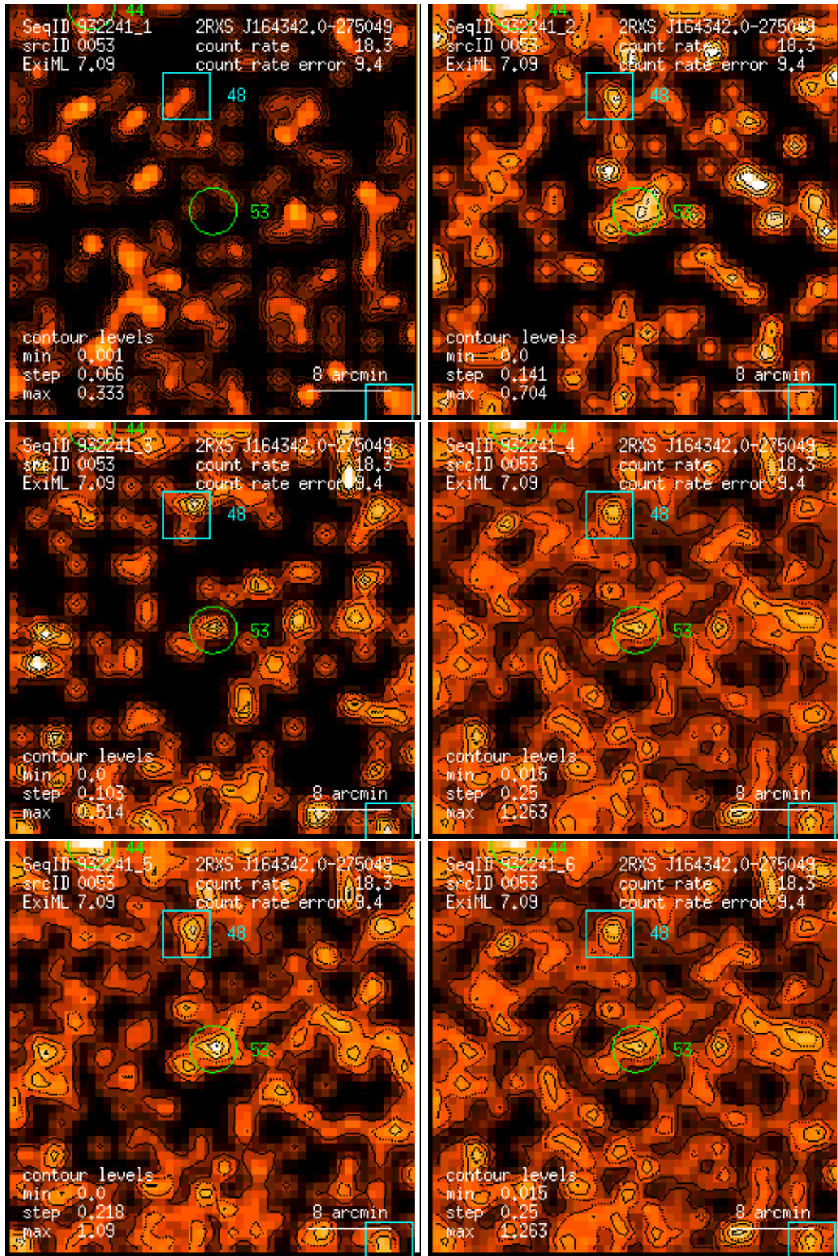
Figure 53: RASS 932241: detection 0053: band rate images, Gaussian filter: (1) PSPC channels 11 – 41, (2) 52 – 90, (3) 91 – 201, (4) 11 – 235, (5) 52 – 201, (6) 11 – 201. Broad band rates in counts/ks. Band rate contour levels in counts/ks/arcmin 2 .
