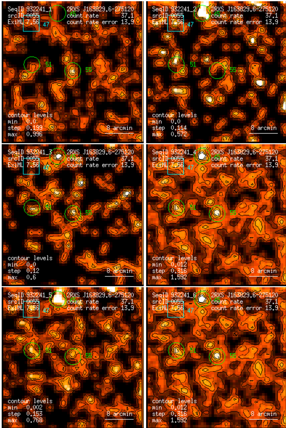
Figure 55: RASS 932241: detection 0055: band rate images, Gaussian filter: (1) PSPC channels 11 – 41, (2) 52 – 90, (3) 91 – 201, (4) 11 – 235, (5) 52 – 201, (6) 11 – 201. Broad band rates in counts/ks. Band rate contour levels in counts/ks/arcmin 2 .
