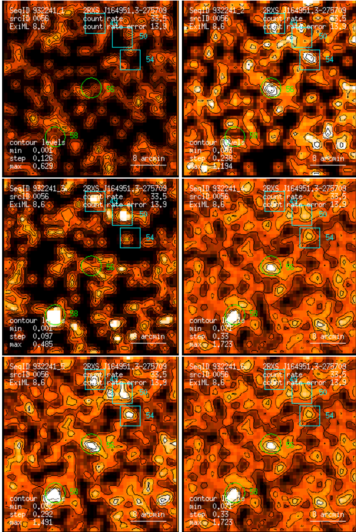
Figure 56: RASS 932241: detection 0056: band rate images, Gaussian filter: (1) PSPC channels 11 – 41, (2) 52 – 90, (3) 91 – 201, (4) 11 – 235, (5) 52 – 201, (6) 11 – 201. Broad band rates in counts/ks. Band rate contour levels in counts/ks/arcmin 2 .
