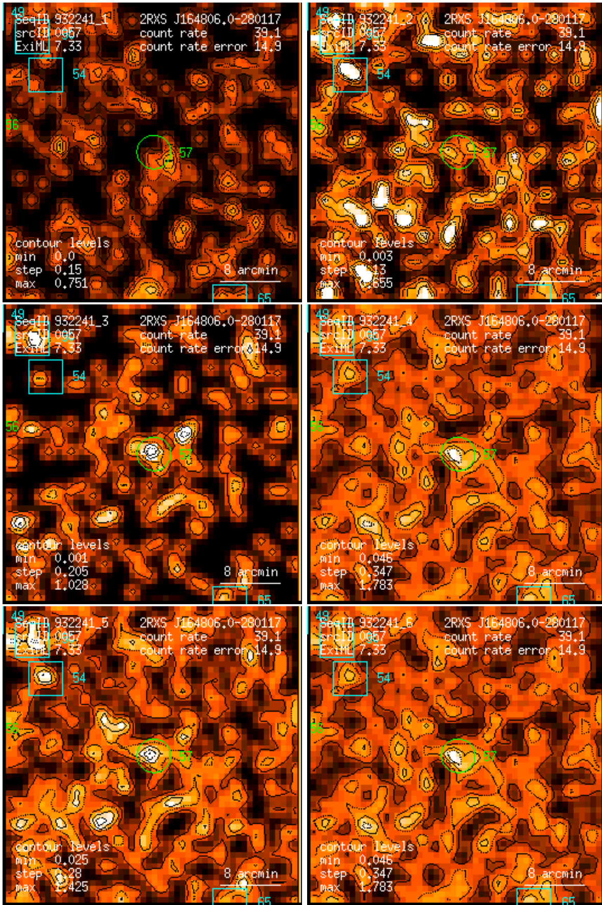
Figure 57: RASS 932241: detection 0057: band rate images, Gaussian filter: (1) PSPC channels 11 – 41, (2) 52 – 90, (3) 91 – 201, (4) 11 – 235, (5) 52 – 201, (6) 11 – 201. Broad band rates in counts/ks. Band rate contour levels in counts/ks/arcmin 2 .
