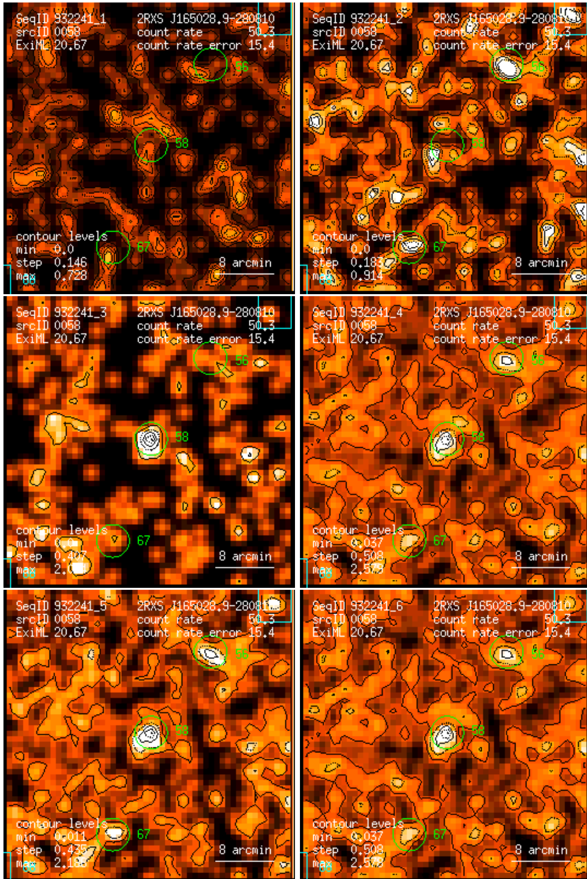
Figure 58: RASS 932241: detection 0058: band rate images, Gaussian filter: (1) PSPC channels 11 – 41, (2) 52 – 90, (3) 91 – 201, (4) 11 – 235, (5) 52 – 201, (6) 11 – 201. Broad band rates in counts/ks. Band rate contour levels in counts/ks/arcmin 2 .
