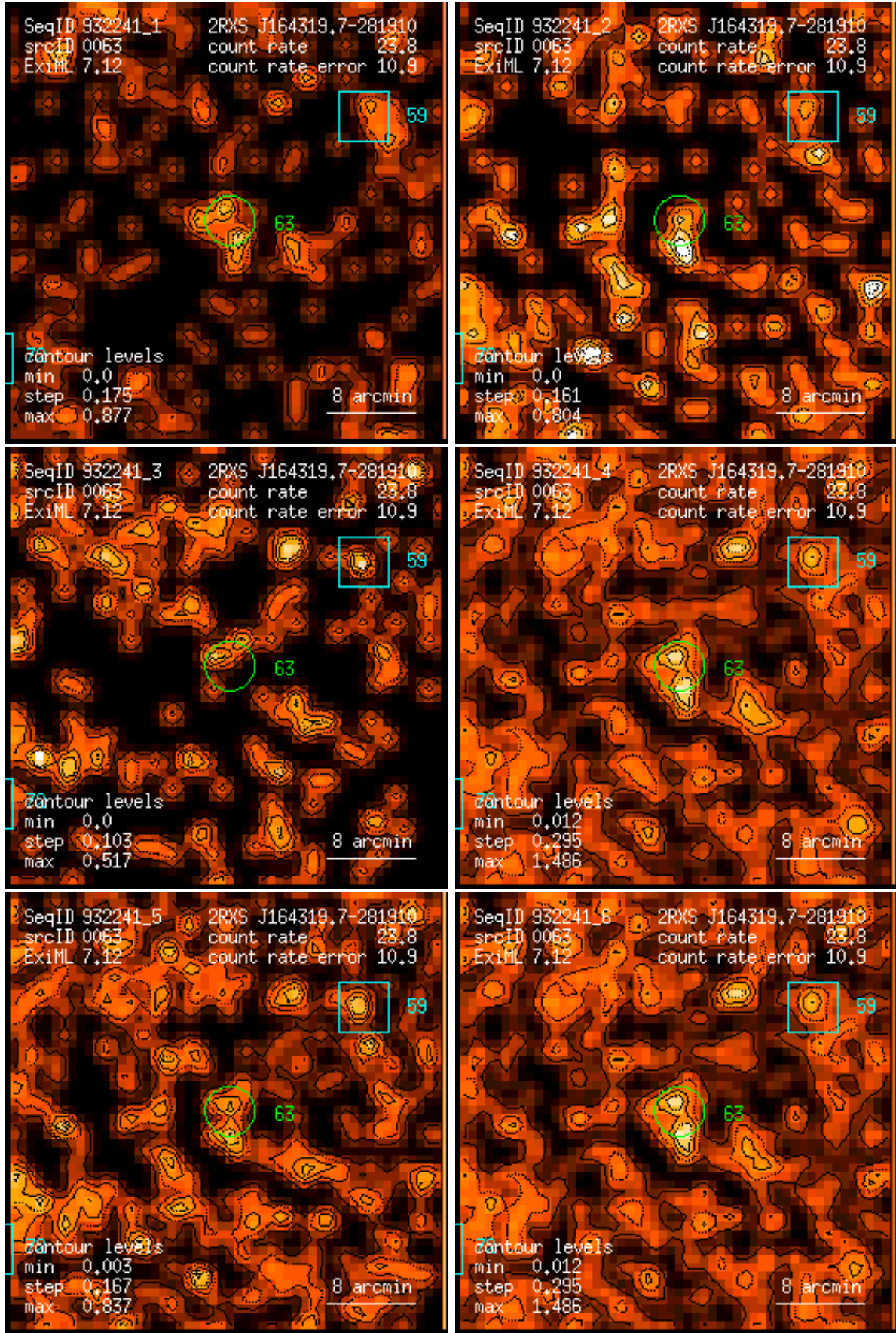
Figure 63: RASS 932241: detection 0063: band rate images, Gaussian filter: (1) PSPC channels 11 – 41, (2) 52 – 90, (3) 91 – 201, (4) 11 – 235, (5) 52 – 201, (6) 11 – 201. Broad band rates in counts/ks. Band rate contour levels in counts/ks/arcmin 2 .
