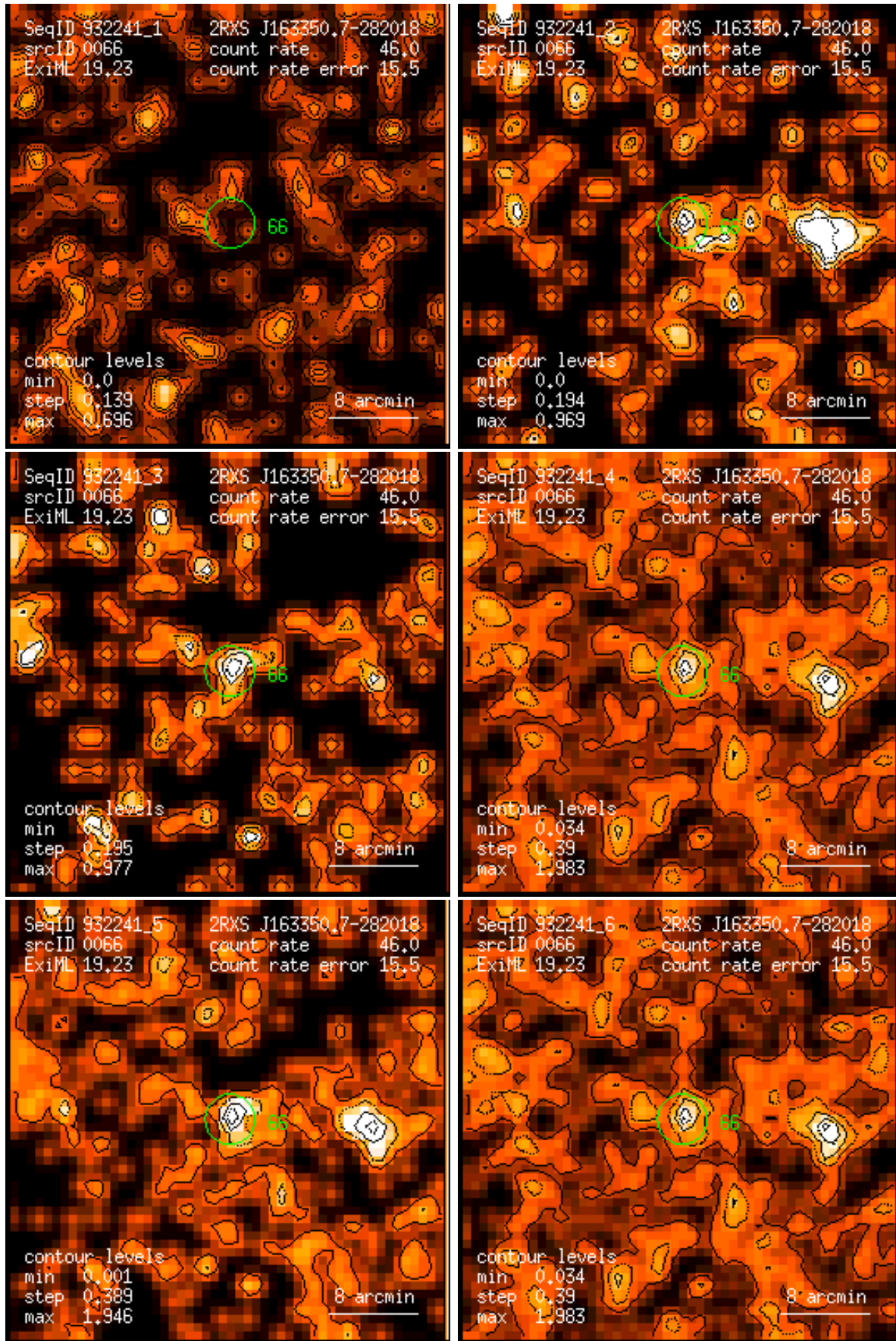
Figure 66: RASS 932241: detection 0066: band rate images, Gaussian filter: (1) PSPC channels 11 – 41, (2) 52 – 90, (3) 91 – 201, (4) 11 – 235, (5) 52 – 201, (6) 11 – 201. Broad band rates in counts/ks. Band rate contour levels in counts/ks/arcmin 2 .
