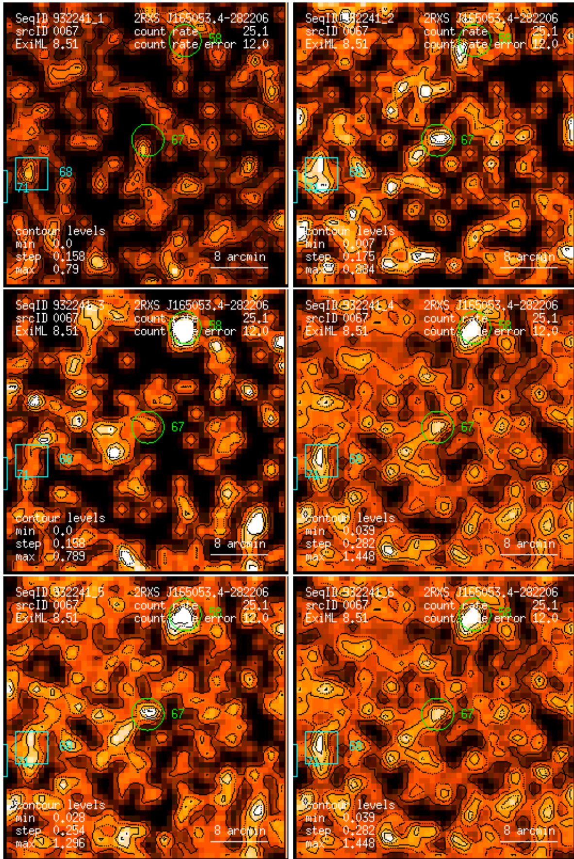
Figure 67: RASS 932241: detection 0067: band rate images, Gaussian filter: (1) PSPC channels 11 – 41, (2) 52 – 90, (3) 91 – 201, (4) 11 – 235, (5) 52 – 201, (6) 11 – 201. Broad band rates in counts/ks. Band rate contour levels in counts/ks/arcmin 2 .
