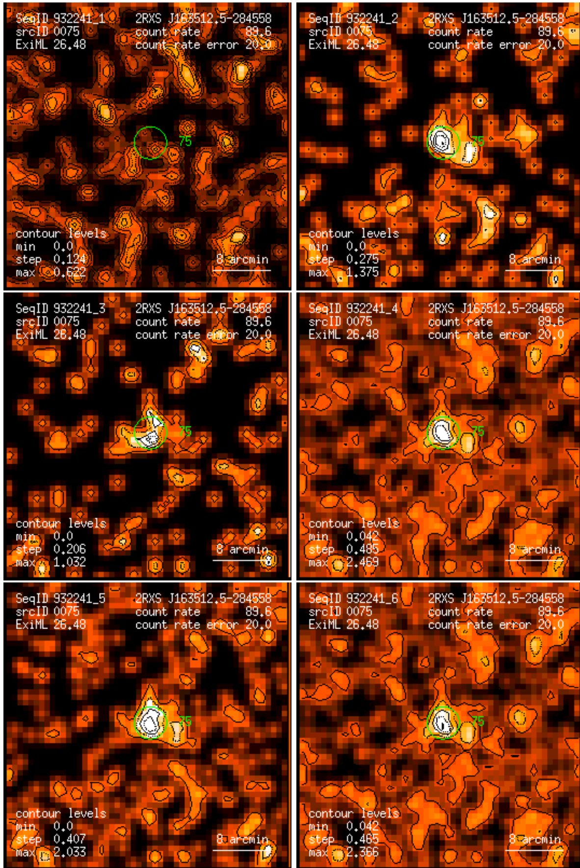
Figure 75: RASS 932241: detection 0075: band rate images, Gaussian filter: (1) PSPC channels 11 – 41, (2) 52 – 90, (3) 91 – 201, (4) 11 – 235, (5) 52 – 201, (6) 11 – 201. Broad band rates in counts/ks. Band rate contour levels in counts/ks/arcmin 2 .
