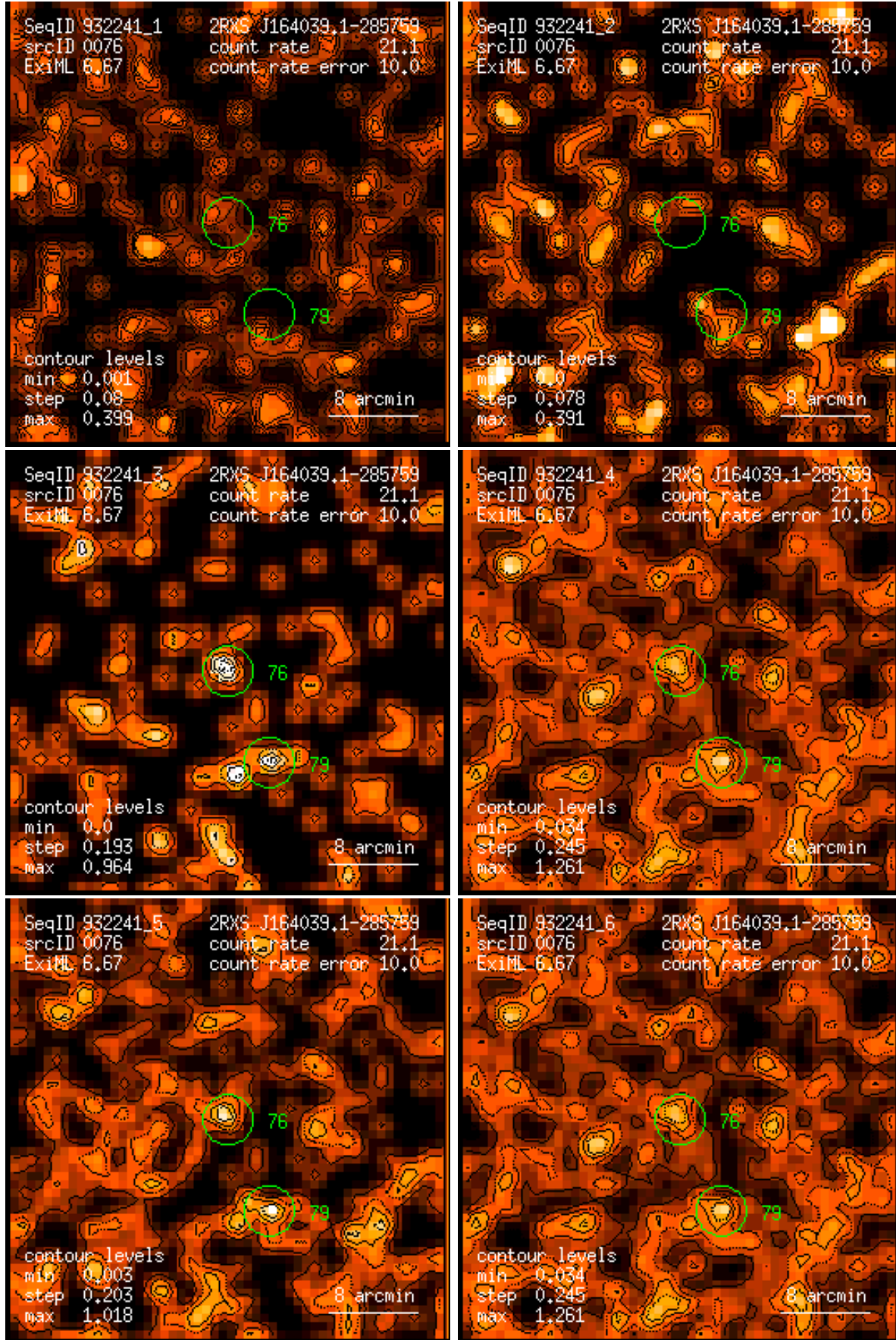
Figure 76: RASS 932241: detection 0076: band rate images, Gaussian filter: (1) PSPC channels 11 – 41, (2) 52 – 90, (3) 91 – 201, (4) 11 – 235, (5) 52 – 201, (6) 11 – 201. Broad band rates in counts/ks. Band rate contour levels in counts/ks/arcmin 2 .
