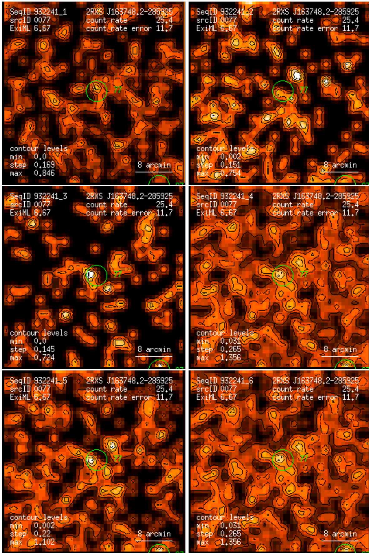
Figure 77: RASS 932241: detection 0077: band rate images, Gaussian filter: (1) PSPC channels 11 – 41, (2) 52 – 90, (3) 91 – 201, (4) 11 – 235, (5) 52 – 201, (6) 11 – 201. Broad band rates in counts/ks. Band rate contour levels in counts/ks/arcmin 2 .
