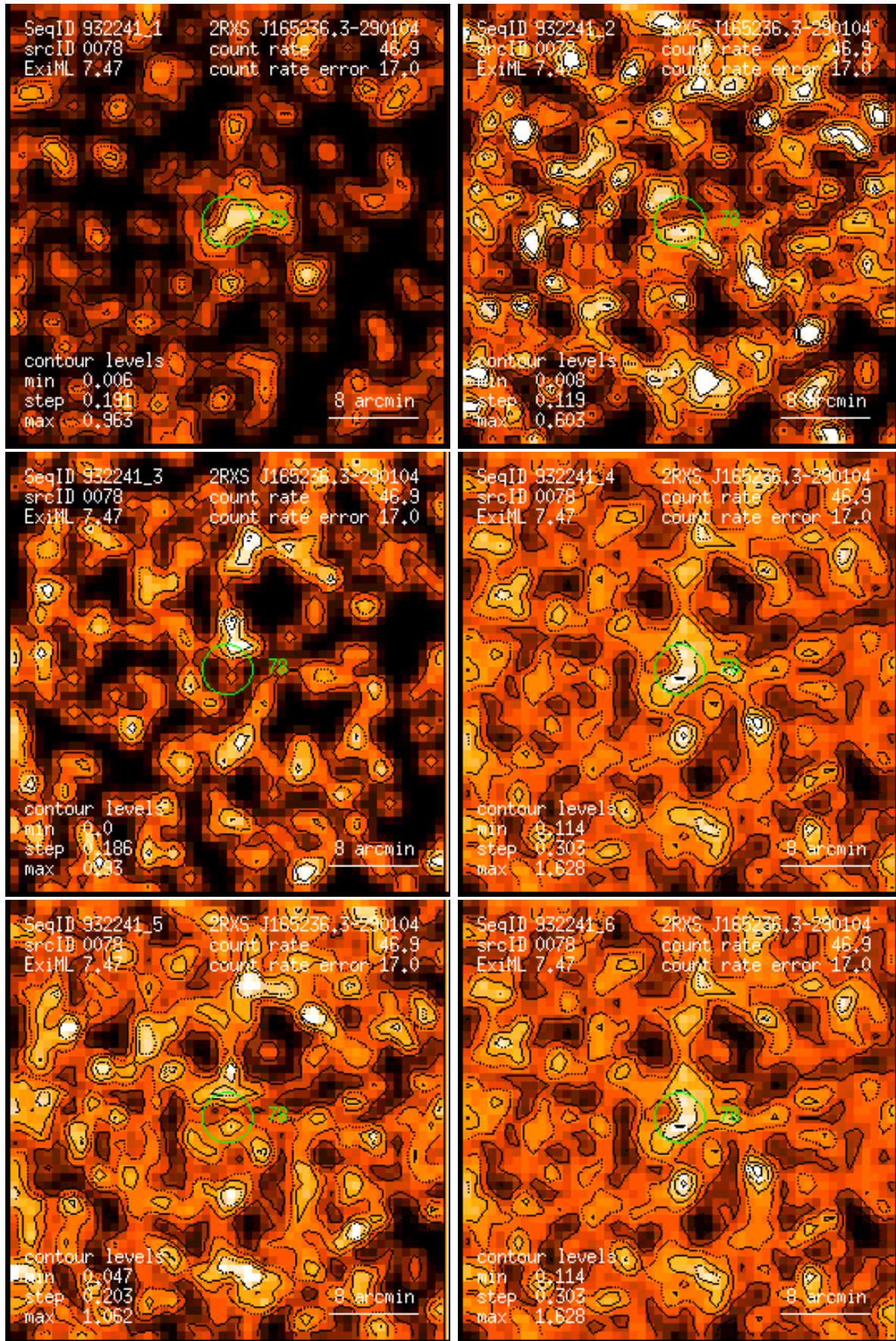
Figure 78: RASS 932241: detection 0078: band rate images, Gaussian filter: (1) PSPC channels 11 – 41, (2) 52 – 90, (3) 91 – 201, (4) 11 – 235, (5) 52 – 201, (6) 11 – 201. Broad band rates in counts/ks. Band rate contour levels in counts/ks/arcmin 2 .
