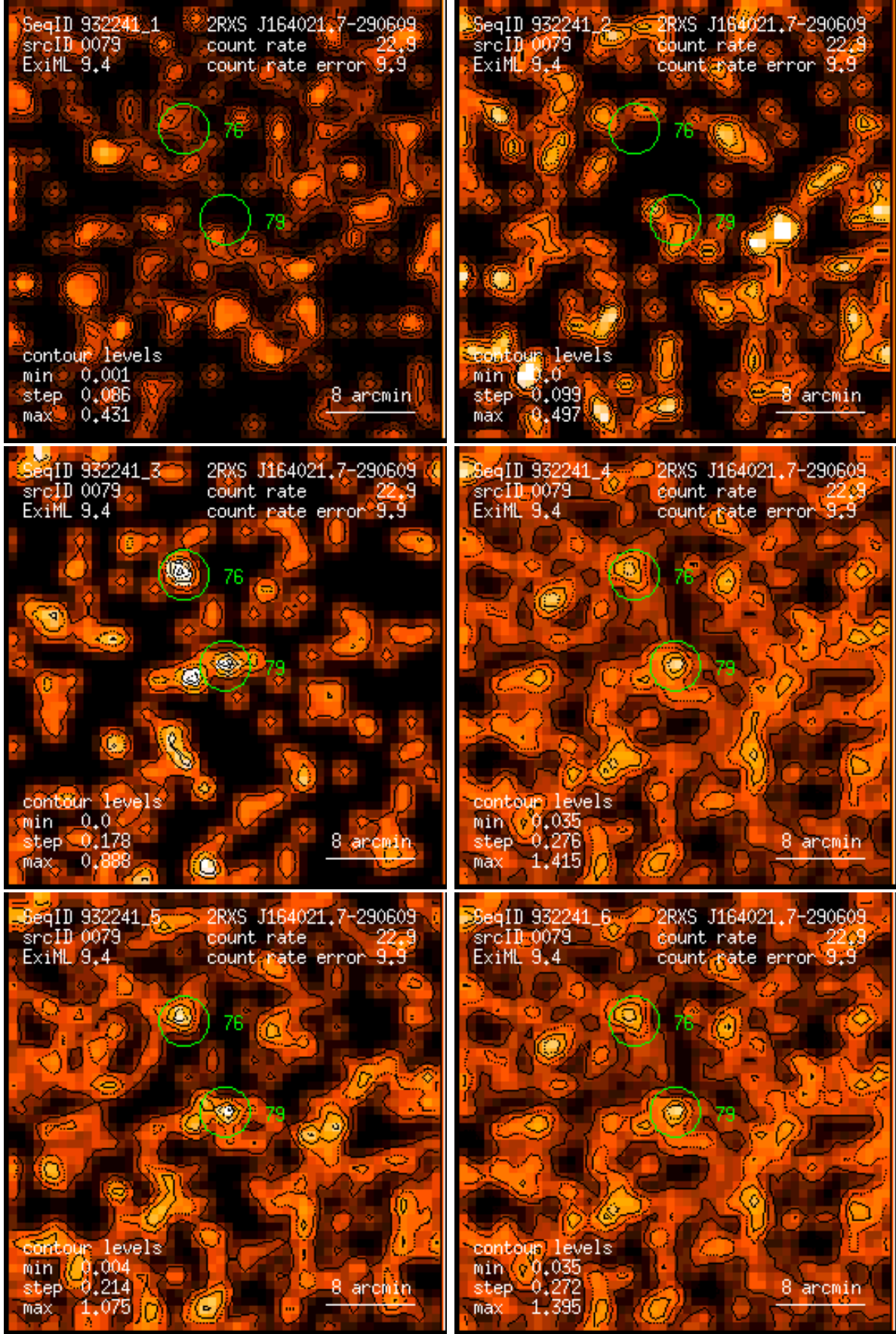
Figure 79: RASS 932241: detection 0079: band rate images, Gaussian filter: (1) PSPC channels 11 – 41, (2) 52 – 90, (3) 91 – 201, (4) 11 – 235, (5) 52 – 201, (6) 11 – 201. Broad band rates in counts/ks. Band rate contour levels in counts/ks/arcmin 2 .
