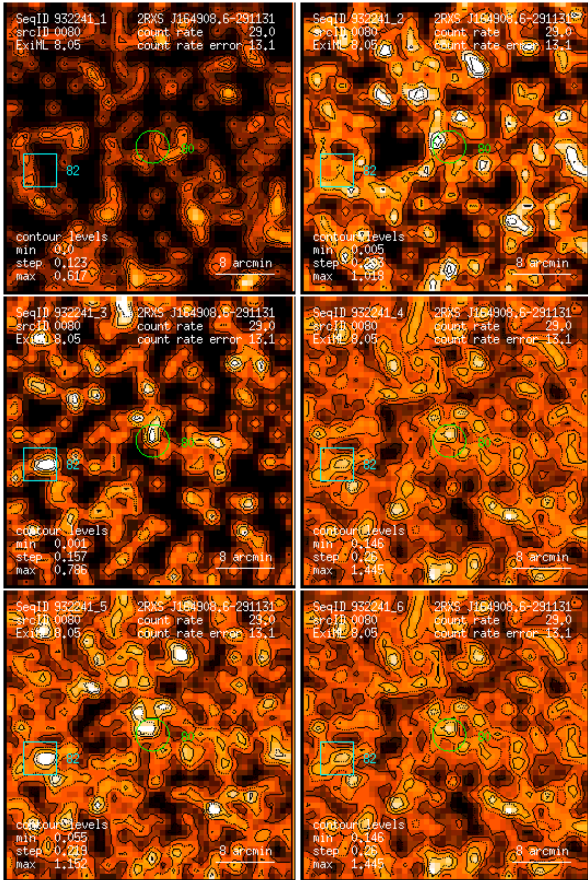
Figure 80: RASS 932241: detection 0080: band rate images, Gaussian filter: (1) PSPC channels 11 – 41, (2) 52 – 90, (3) 91 – 201, (4) 11 – 235, (5) 52 – 201, (6) 11 – 201. Broad band rates in counts/ks. Band rate contour levels in counts/ks/arcmin 2 .
