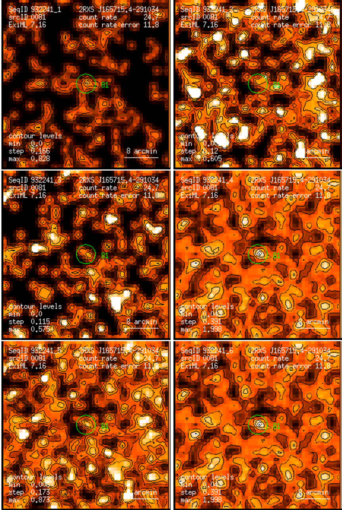
Figure 81: RASS 932241: detection 0081: band rate images, Gaussian filter: (1) PSPC channels 11 – 41, (2) 52 – 90, (3) 91 – 201, (4) 11 – 235, (5) 52 – 201, (6) 11 – 201. Broad band rates in counts/ks. Band rate contour levels in counts/ks/arcmin 2 .
