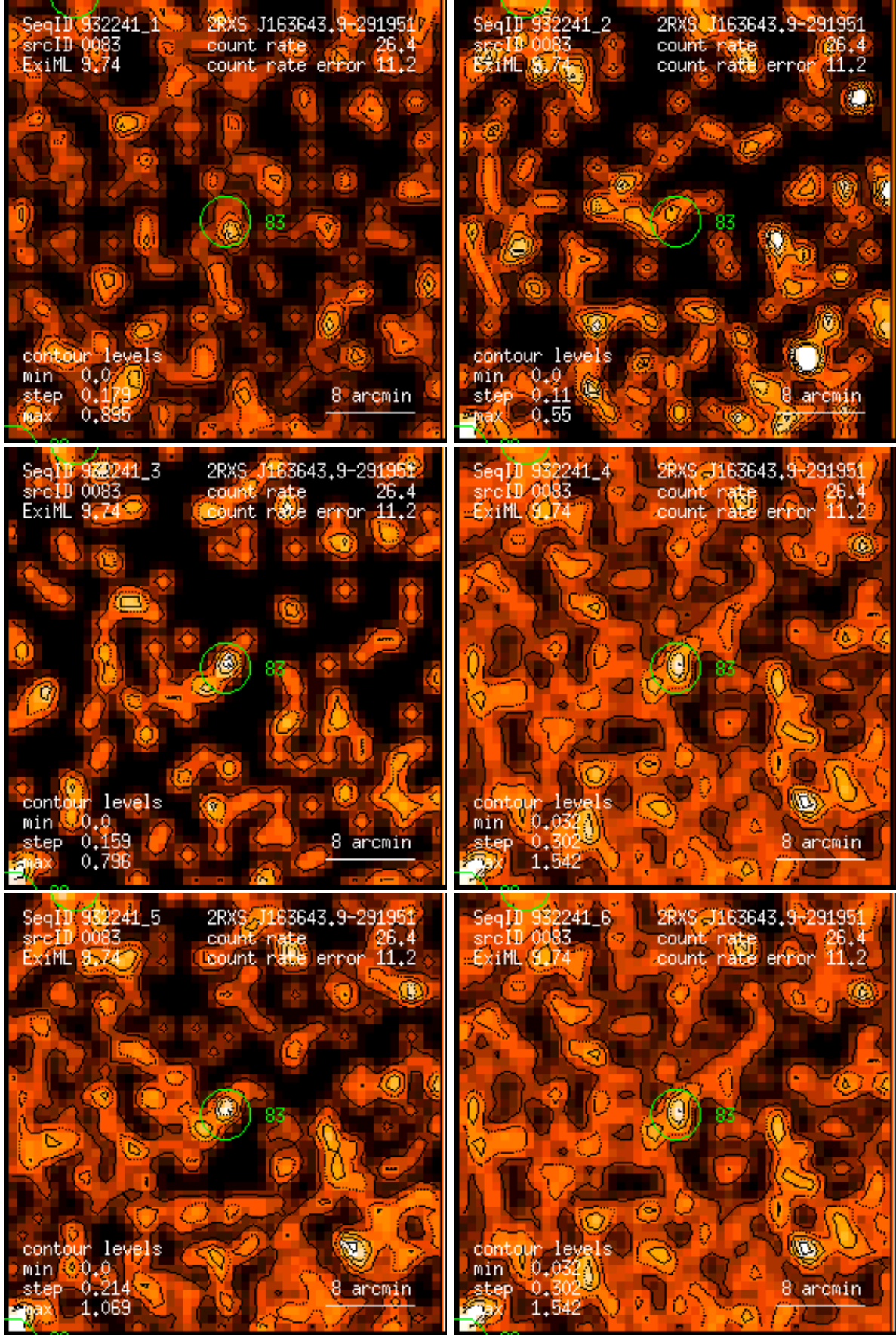
Figure 83: RASS 932241: detection 0083: band rate images, Gaussian filter: (1) PSPC channels 11 – 41, (2) 52 – 90, (3) 91 – 201, (4) 11 – 235, (5) 52 – 201, (6) 11 – 201. Broad band rates in counts/ks. Band rate contour levels in counts/ks/arcmin 2 .
