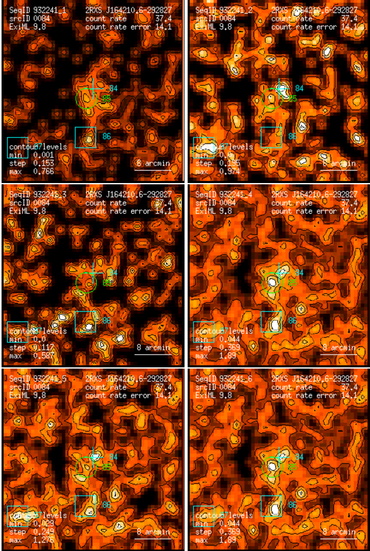
Figure 84: RASS 932241: detection 0084: band rate images, Gaussian filter: (1) PSPC channels 11 – 41, (2) 52 – 90, (3) 91 – 201, (4) 11 – 235, (5) 52 – 201, (6) 11 – 201. Broad band rates in counts/ks. Band rate contour levels in counts/ks/arcmin 2 .
