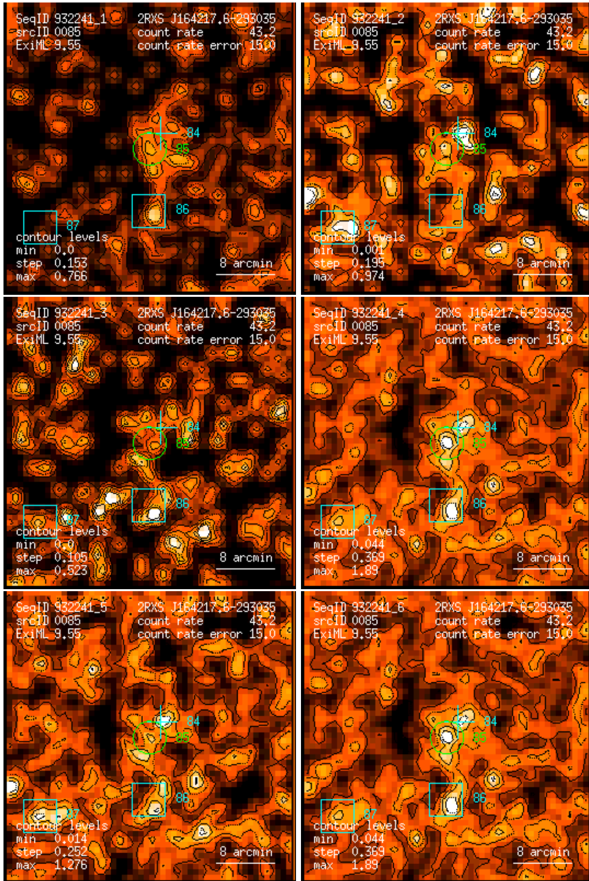
Figure 85: RASS 932241: detection 0085: band rate images, Gaussian filter: (1) PSPC channels 11 – 41, (2) 52 – 90, (3) 91 – 201, (4) 11 – 235, (5) 52 – 201, (6) 11 – 201. Broad band rates in counts/ks. Band rate contour levels in counts/ks/arcmin 2 .
