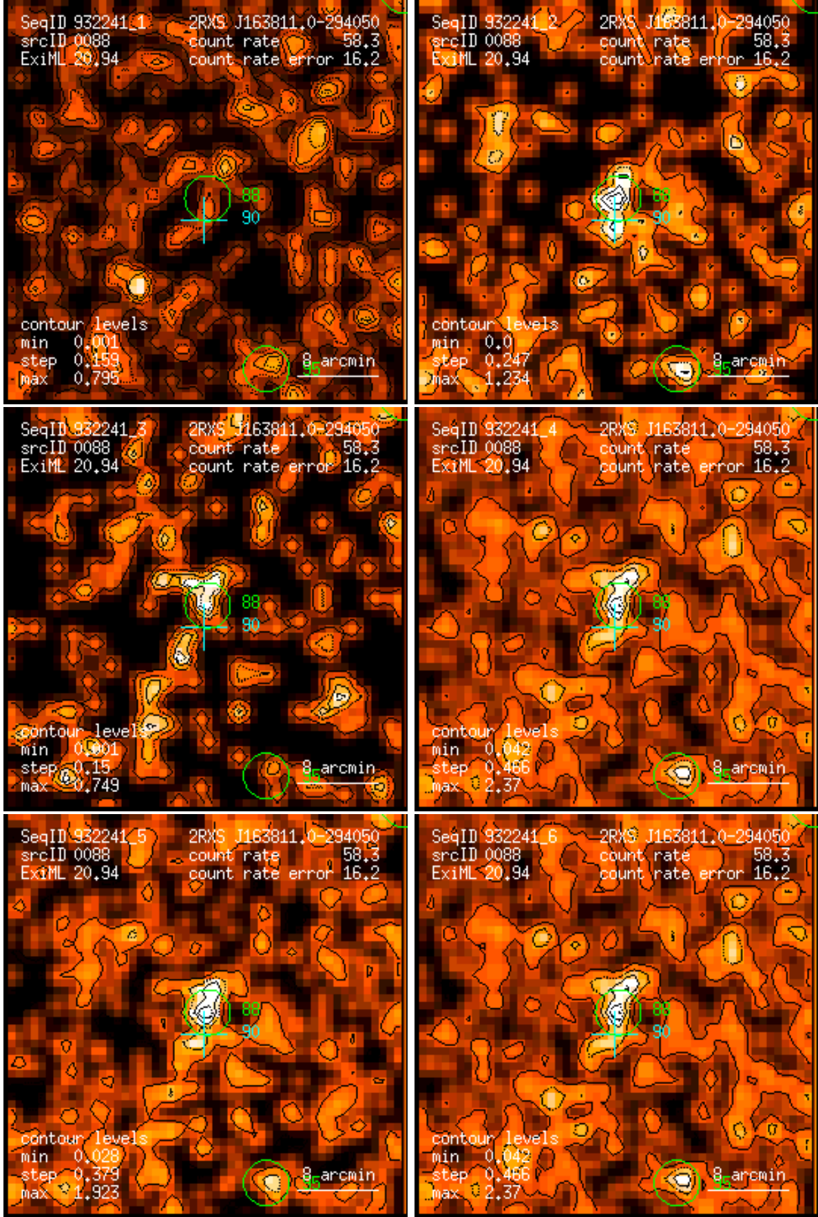
Figure 88: RASS 932241: detection 0088: band rate images, Gaussian filter: (1) PSPC channels 11 – 41, (2) 52 – 90, (3) 91 – 201, (4) 11 – 235, (5) 52 – 201, (6) 11 – 201. Broad band rates in counts/ks. Band rate contour levels in counts/ks/arcmin 2 .
