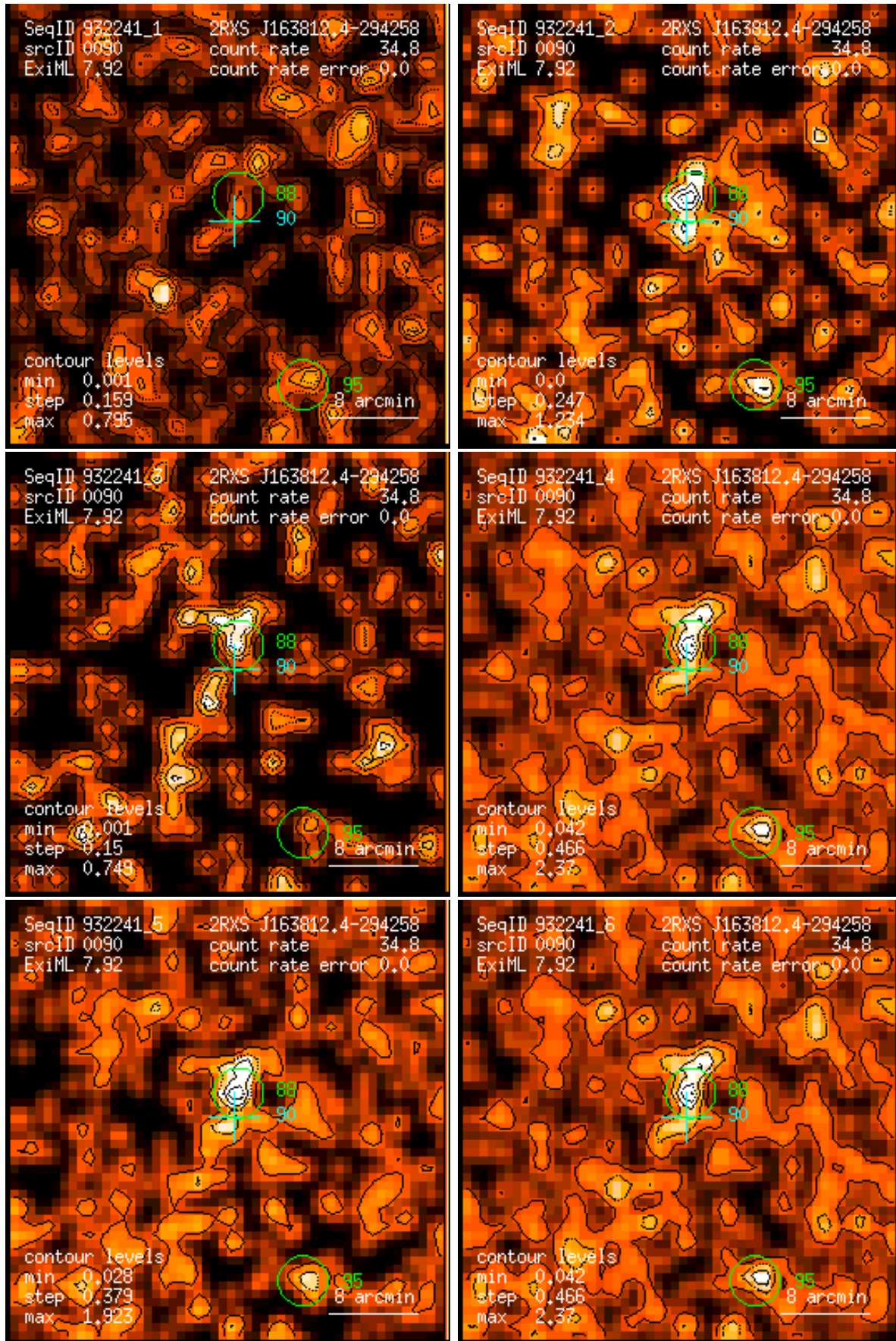
Figure 90: RASS 932241: detection 0090: band rate images, Gaussian filter: (1) PSPC channels 11 – 41, (2) 52 – 90, (3) 91 – 201, (4) 11 – 235, (5) 52 – 201, (6) 11 – 201. Broad band rates in counts/ks. Band rate contour levels in counts/ks/arcmin 2 .
