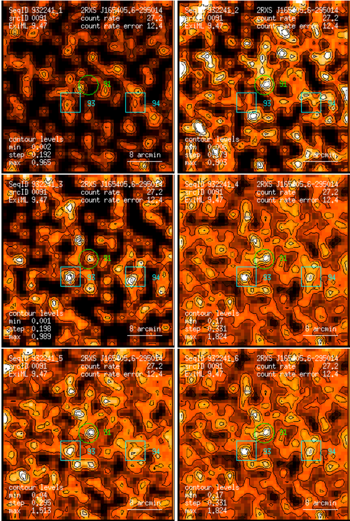
Figure 91: RASS 932241: detection 0091: band rate images, Gaussian filter: (1) PSPC channels 11 – 41, (2) 52 – 90, (3) 91 – 201, (4) 11 – 235, (5) 52 – 201, (6) 11 – 201. Broad band rates in counts/ks. Band rate contour levels in counts/ks/arcmin 2 .
