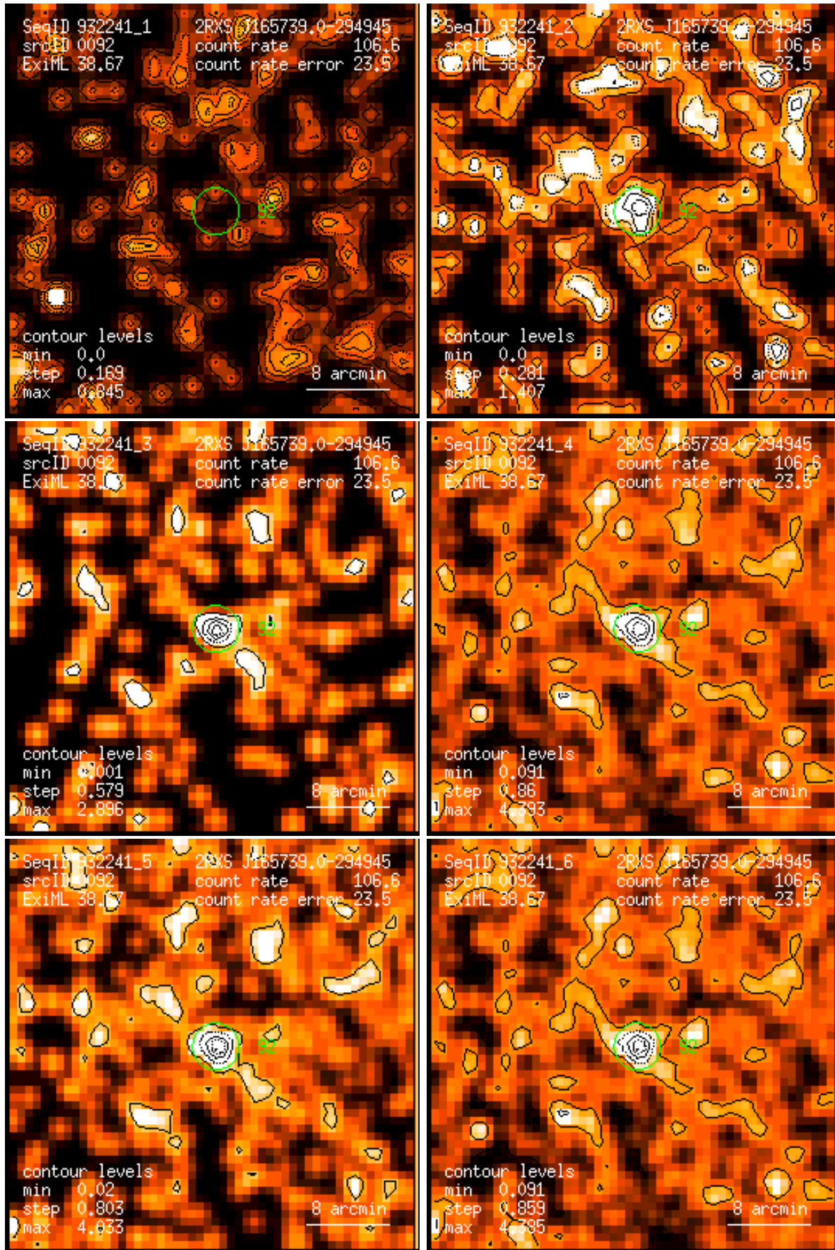
Figure 92: RASS 932241: detection 0092: band rate images, Gaussian filter: (1) PSPC channels 11 – 41, (2) 52 – 90, (3) 91 – 201, (4) 11 – 235, (5) 52 – 201, (6) 11 – 201. Broad band rates in counts/ks. Band rate contour levels in counts/ks/arcmin 2 .
