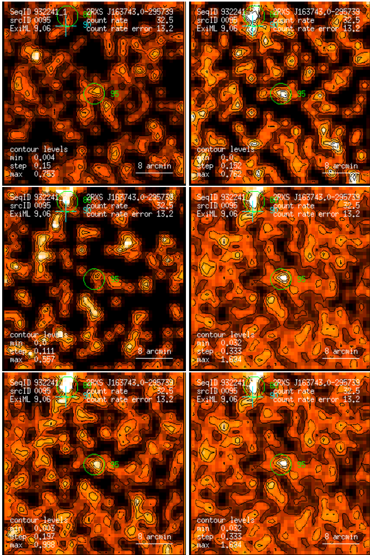
Figure 95: RASS 932241: detection 0095: band rate images, Gaussian filter: (1) PSPC channels 11 – 41, (2) 52 – 90, (3) 91 – 201, (4) 11 – 235, (5) 52 – 201, (6) 11 – 201. Broad band rates in counts/ks. Band rate contour levels in counts/ks/arcmin 2 .
