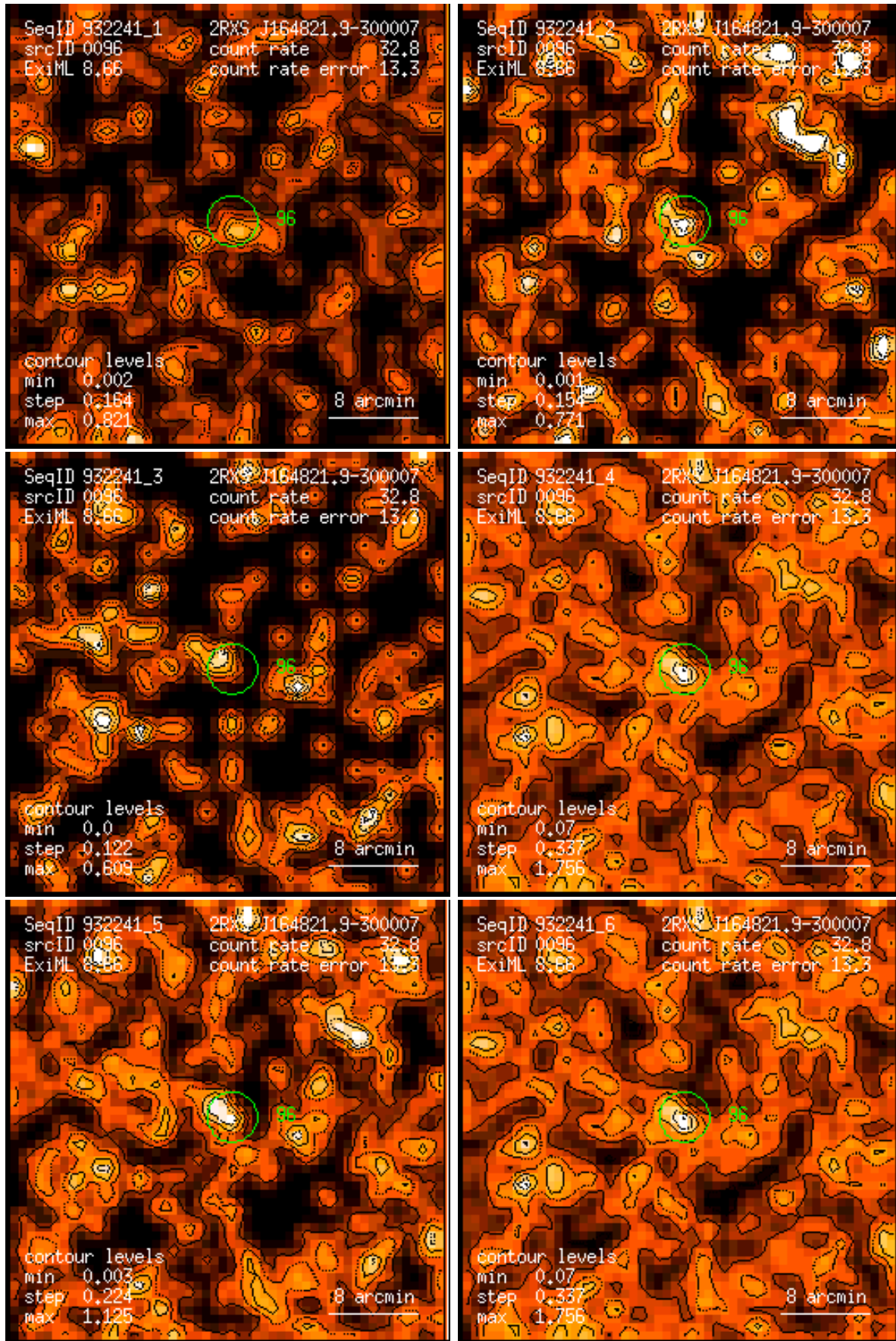
Figure 96: RASS 932241: detection 0096: band rate images, Gaussian filter: (1) PSPC channels 11 – 41, (2) 52 – 90, (3) 91 – 201, (4) 11 – 235, (5) 52 – 201, (6) 11 – 201. Broad band rates in counts/ks. Band rate contour levels in counts/ks/arcmin 2 .
