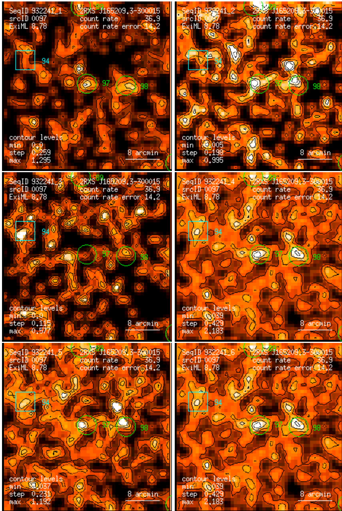
Figure 97: RASS 932241: detection 0097: band rate images, Gaussian filter: (1) PSPC channels 11 – 41, (2) 52 – 90, (3) 91 – 201, (4) 11 – 235, (5) 52 – 201, (6) 11 – 201. Broad band rates in counts/ks. Band rate contour levels in counts/ks/arcmin 2 .
