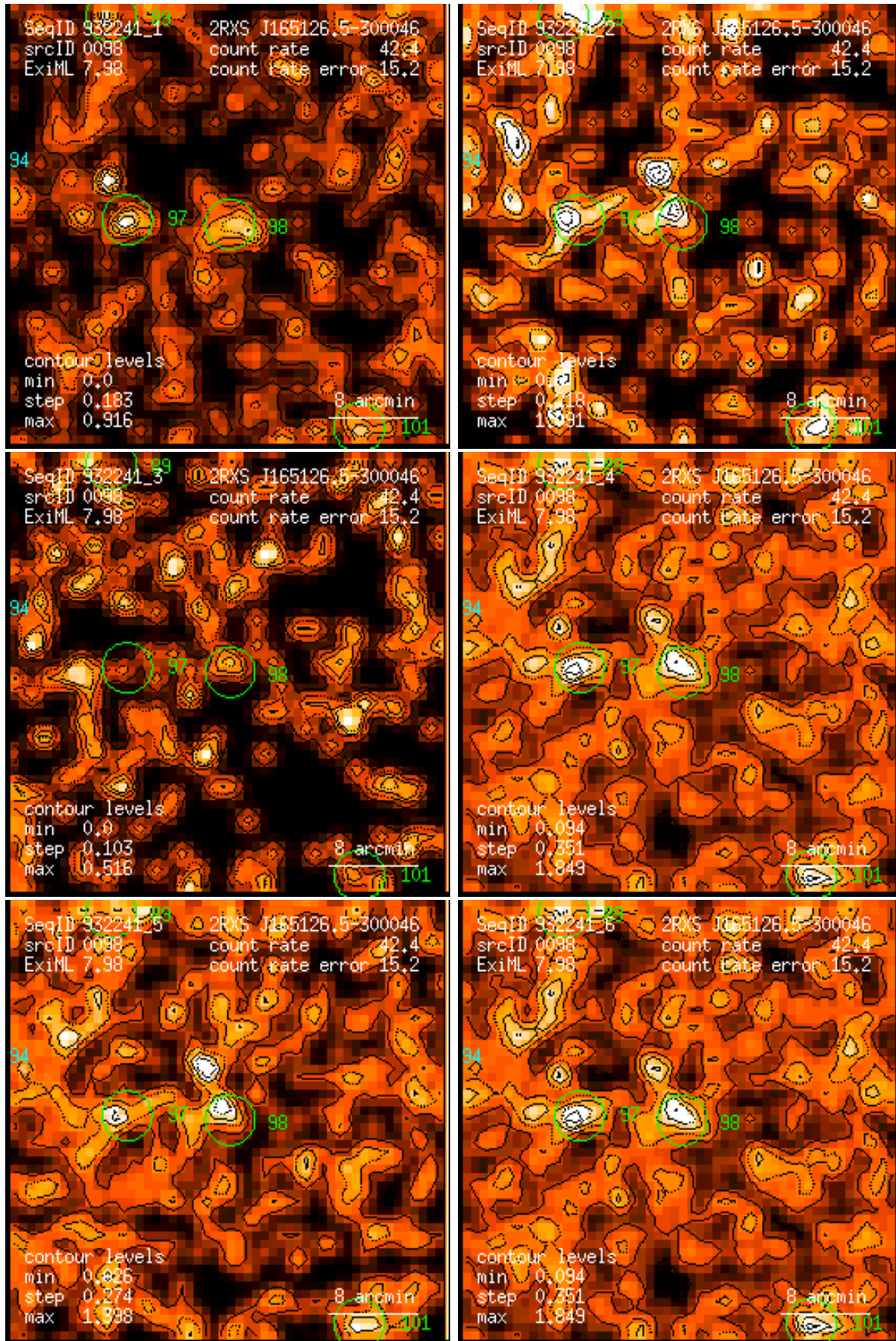
Figure 98: RASS 932241: detection 0098: band rate images, Gaussian filter: (1) PSPC channels 11 – 41, (2) 52 – 90, (3) 91 – 201, (4) 11 – 235, (5) 52 – 201, (6) 11 – 201. Broad band rates in counts/ks. Band rate contour levels in counts/ks/arcmin 2 .
