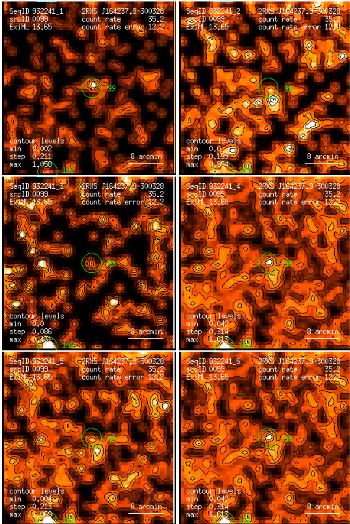
Figure 99: RASS 932241: detection 0099: band rate images, Gaussian filter: (1) PSPC channels 11 – 41, (2) 52 – 90, (3) 91 – 201, (4) 11 – 235, (5) 52 – 201, (6) 11 – 201. Broad band rates in counts/ks. Band rate contour levels in counts/ks/arcmin 2 .
