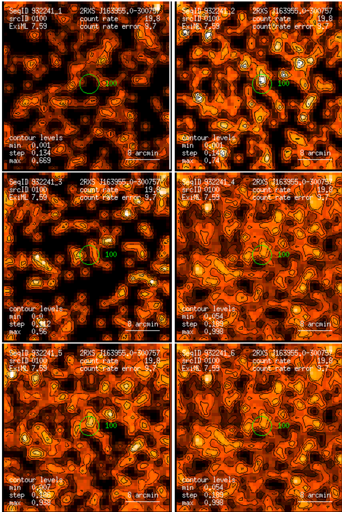
Figure 100: RASS 932241: detection 0100: band rate images, Gaussian filter: (1) PSPC channels 11 – 41, (2) 52 – 90, (3) 91 – 201, (4) 11 – 235, (5) 52 – 201, (6) 11 – 201. Broad band rates in counts/ks. Band rate contour levels in counts/ks/arcmin 2 .
