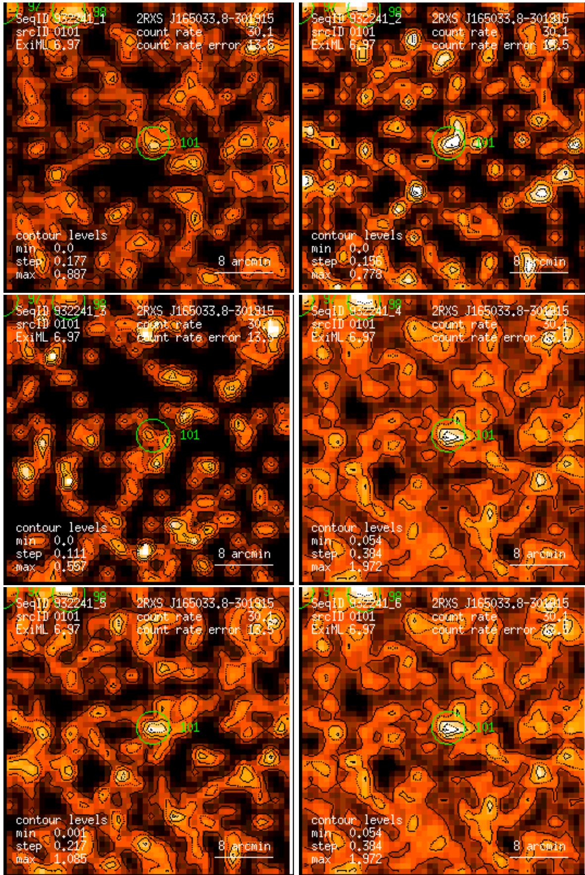
Figure 101: RASS 932241: detection 0101: band rate images, Gaussian filter: (1) PSPC channels 11 – 41, (2) 52 – 90, (3) 91 – 201, (4) 11 – 235, (5) 52 – 201, (6) 11 – 201. Broad band rates in counts/ks. Band rate contour levels in counts/ks/arcmin 2 .
