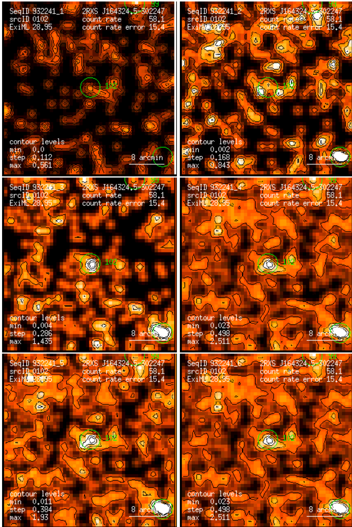
Figure 102: RASS 932241: detection 0102: band rate images, Gaussian filter: (1) PSPC channels 11 – 41, (2) 52 – 90, (3) 91 – 201, (4) 11 – 235, (5) 52 – 201, (6) 11 – 201. Broad band rates in counts/ks. Band rate contour levels in counts/ks/arcmin 2 .
