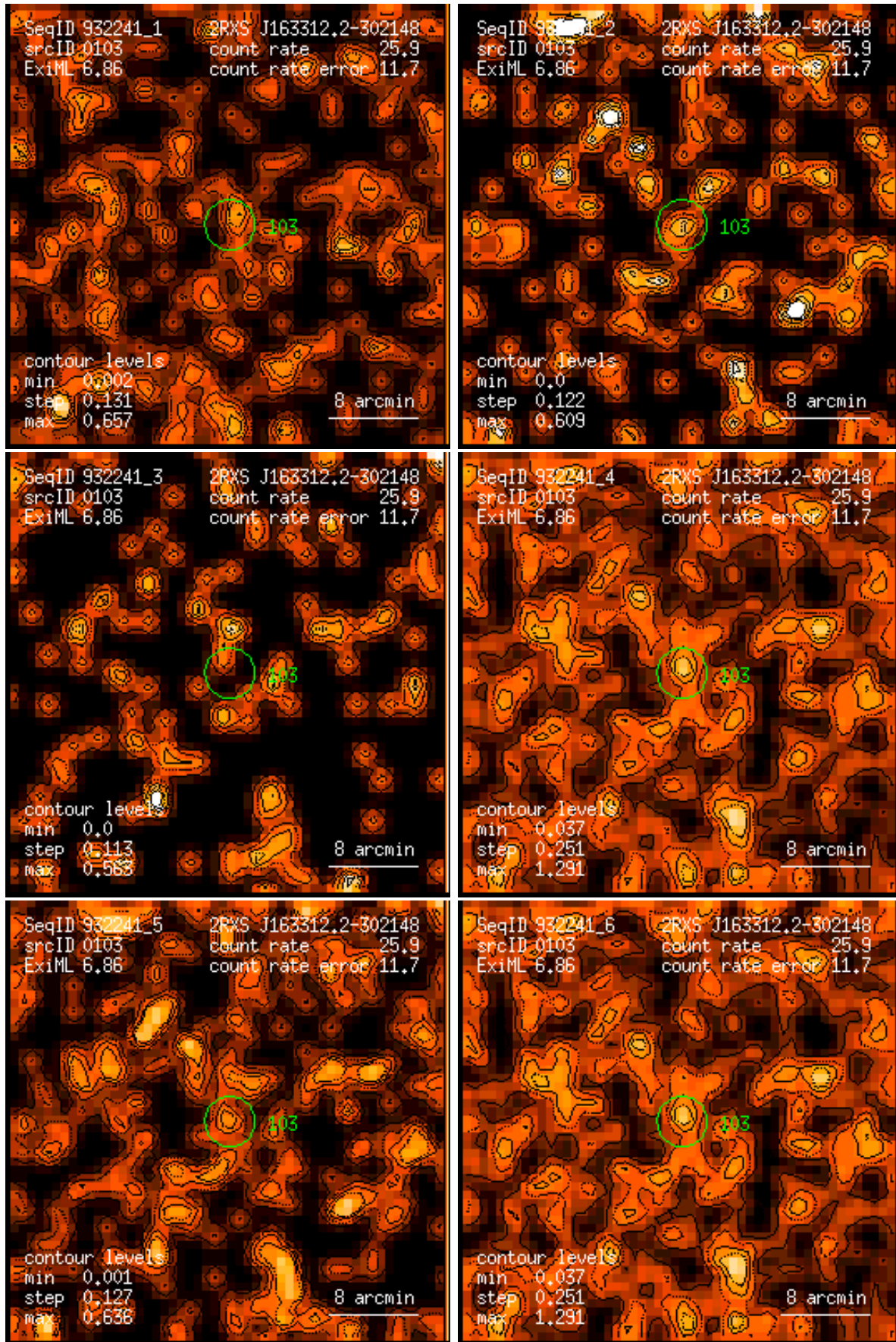
Figure 103: RASS 932241: detection 0103: band rate images, Gaussian filter: (1) PSPC channels 11 – 41, (2) 52 – 90, (3) 91 – 201, (4) 11 – 235, (5) 52 – 201, (6) 11 – 201. Broad band rates in counts/ks. Band rate contour levels in counts/ks/arcmin 2 .
