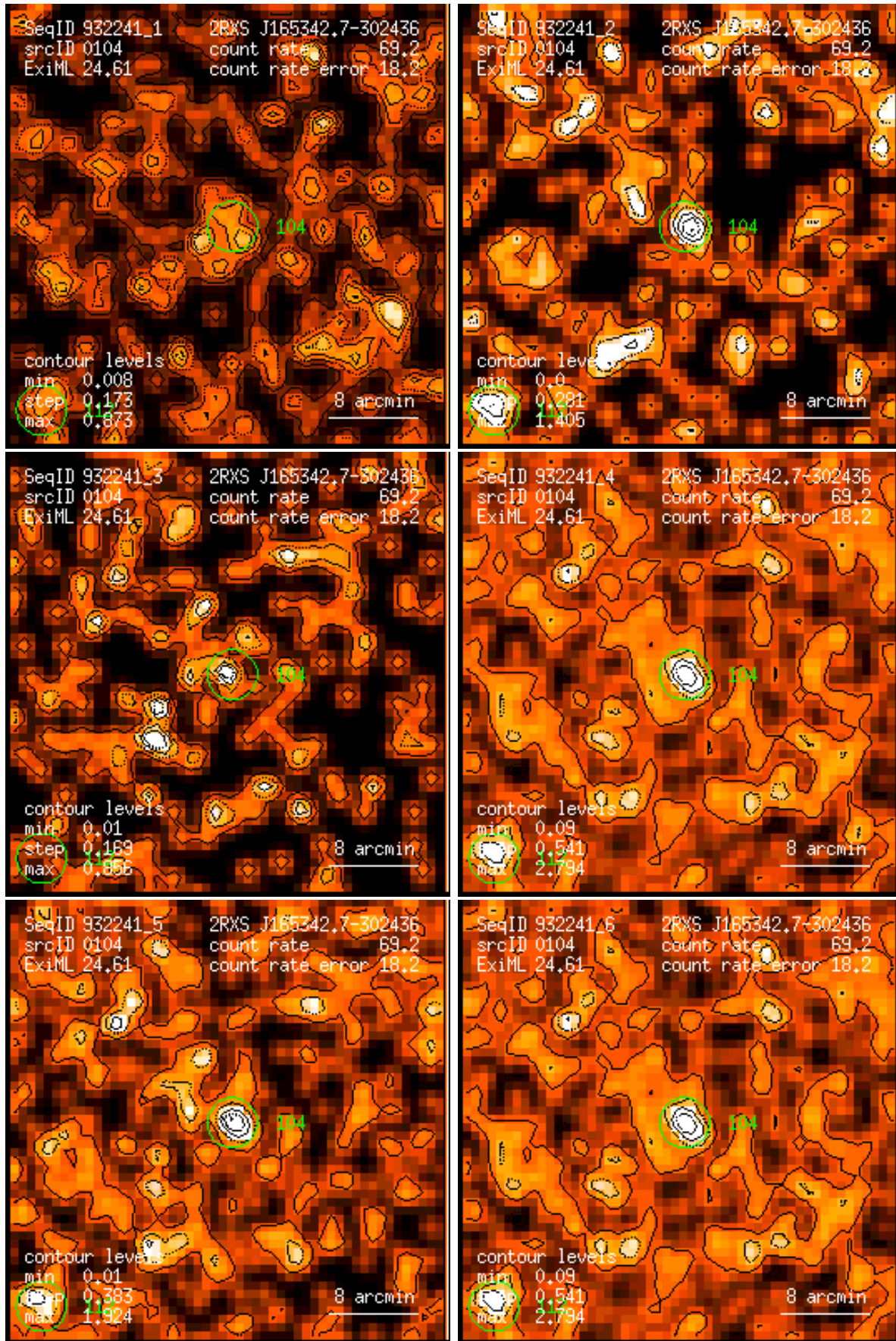
Figure 104: RASS 932241: detection 0104: band rate images, Gaussian filter: (1) PSPC channels 11 – 41, (2) 52 – 90, (3) 91 – 201, (4) 11 – 235, (5) 52 – 201, (6) 11 – 201. Broad band rates in counts/ks. Band rate contour levels in counts/ks/arcmin 2 .
