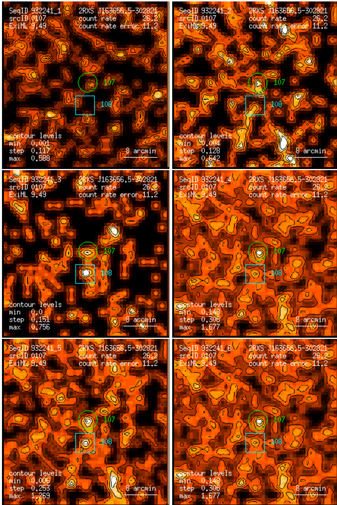
Figure 107: RASS 932241: detection 0107: band rate images, Gaussian filter: (1) PSPC channels 11 – 41, (2) 52 – 90, (3) 91 – 201, (4) 11 – 235, (5) 52 – 201, (6) 11 – 201. Broad band rates in counts/ks. Band rate contour levels in counts/ks/arcmin 2 .
