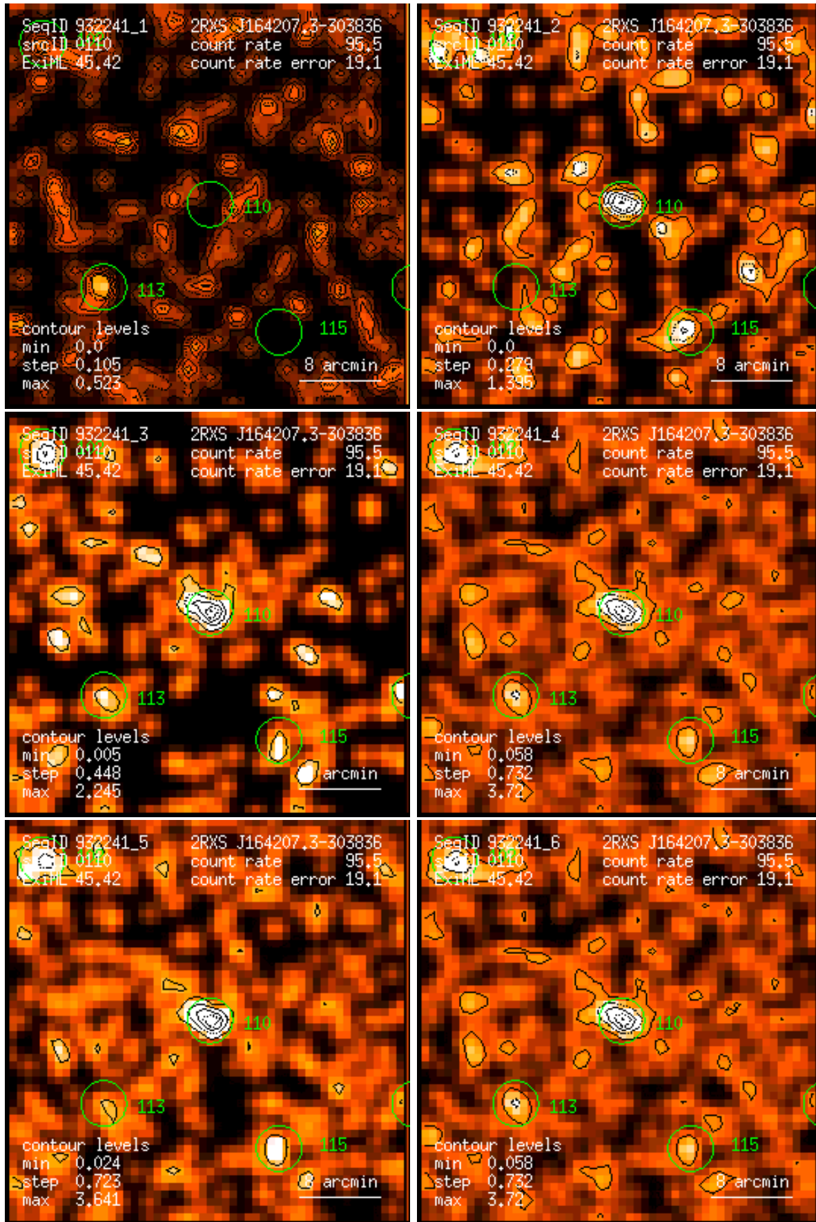
Figure 110: RASS 932241: detection 0110: band rate images, Gaussian filter: (1) PSPC channels 11 – 41, (2) 52 – 90, (3) 91 – 201, (4) 11 – 235, (5) 52 – 201, (6) 11 – 201. Broad band rates in counts/ks. Band rate contour levels in counts/ks/arcmin 2 .
