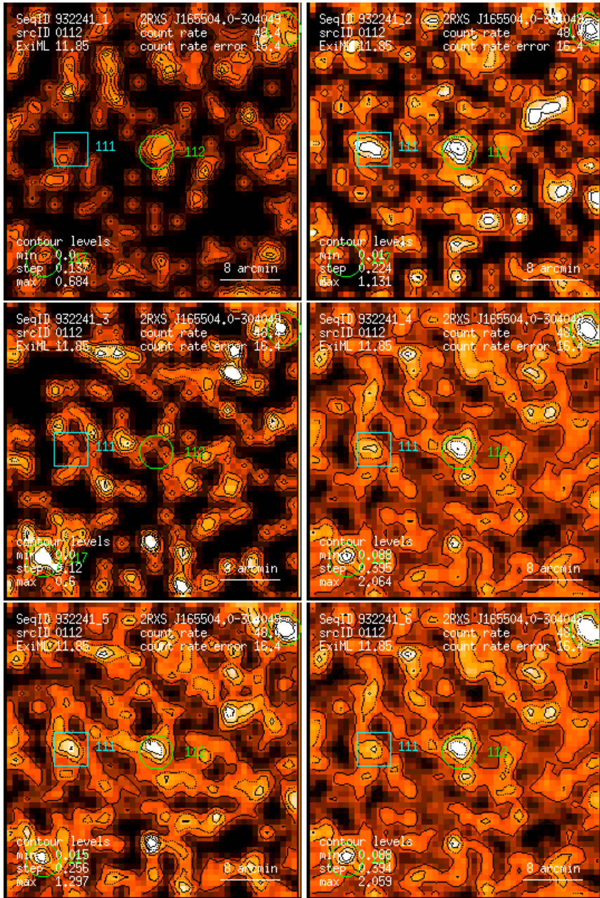
Figure 112: RASS 932241: detection 0112: band rate images, Gaussian filter: (1) PSPC channels 11 – 41, (2) 52 – 90, (3) 91 – 201, (4) 11 – 235, (5) 52 – 201, (6) 11 – 201. Broad band rates in counts/ks. Band rate contour levels in counts/ks/arcmin 2 .
