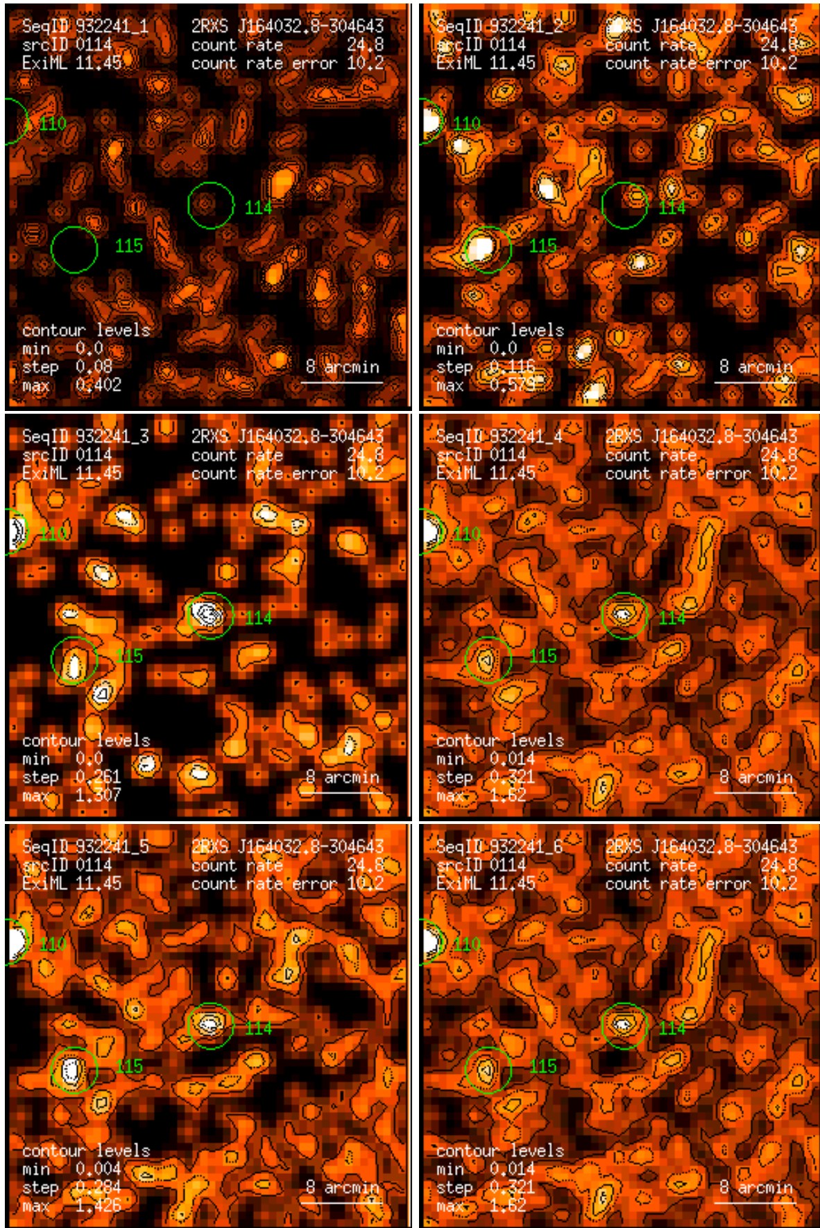
Figure 114: RASS 932241: detection 0114: band rate images, Gaussian filter: (1) PSPC channels 11 – 41, (2) 52 – 90, (3) 91 – 201, (4) 11 – 235, (5) 52 – 201, (6) 11 – 201. Broad band rates in counts/ks. Band rate contour levels in counts/ks/arcmin 2 .
