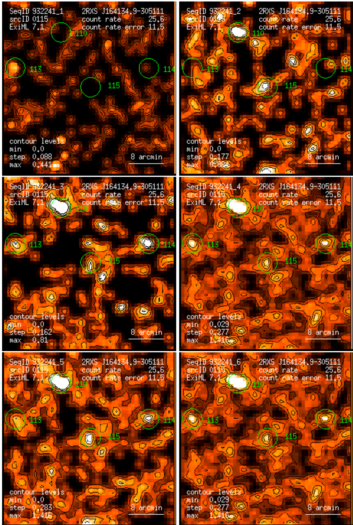
Figure 115: RASS 932241: detection 0115: band rate images, Gaussian filter: (1) PSPC channels 11 – 41, (2) 52 – 90, (3) 91 – 201, (4) 11 – 235, (5) 52 – 201, (6) 11 – 201. Broad band rates in counts/ks. Band rate contour levels in counts/ks/arcmin 2 .
