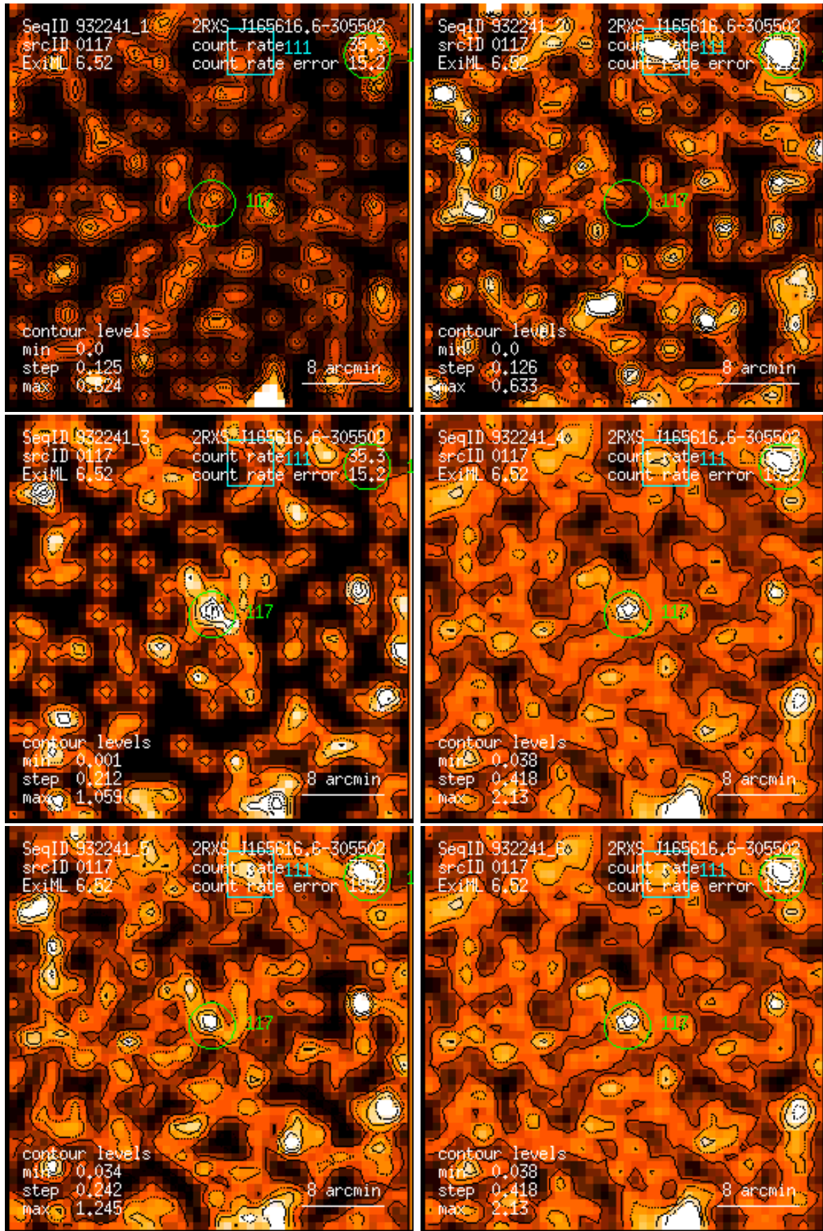
Figure 117: RASS 932241: detection 0117: band rate images, Gaussian filter: (1) PSPC channels 11 – 41, (2) 52 – 90, (3) 91 – 201, (4) 11 – 235, (5) 52 – 201, (6) 11 – 201. Broad band rates in counts/ks. Band rate contour levels in counts/ks/arcmin 2 .
