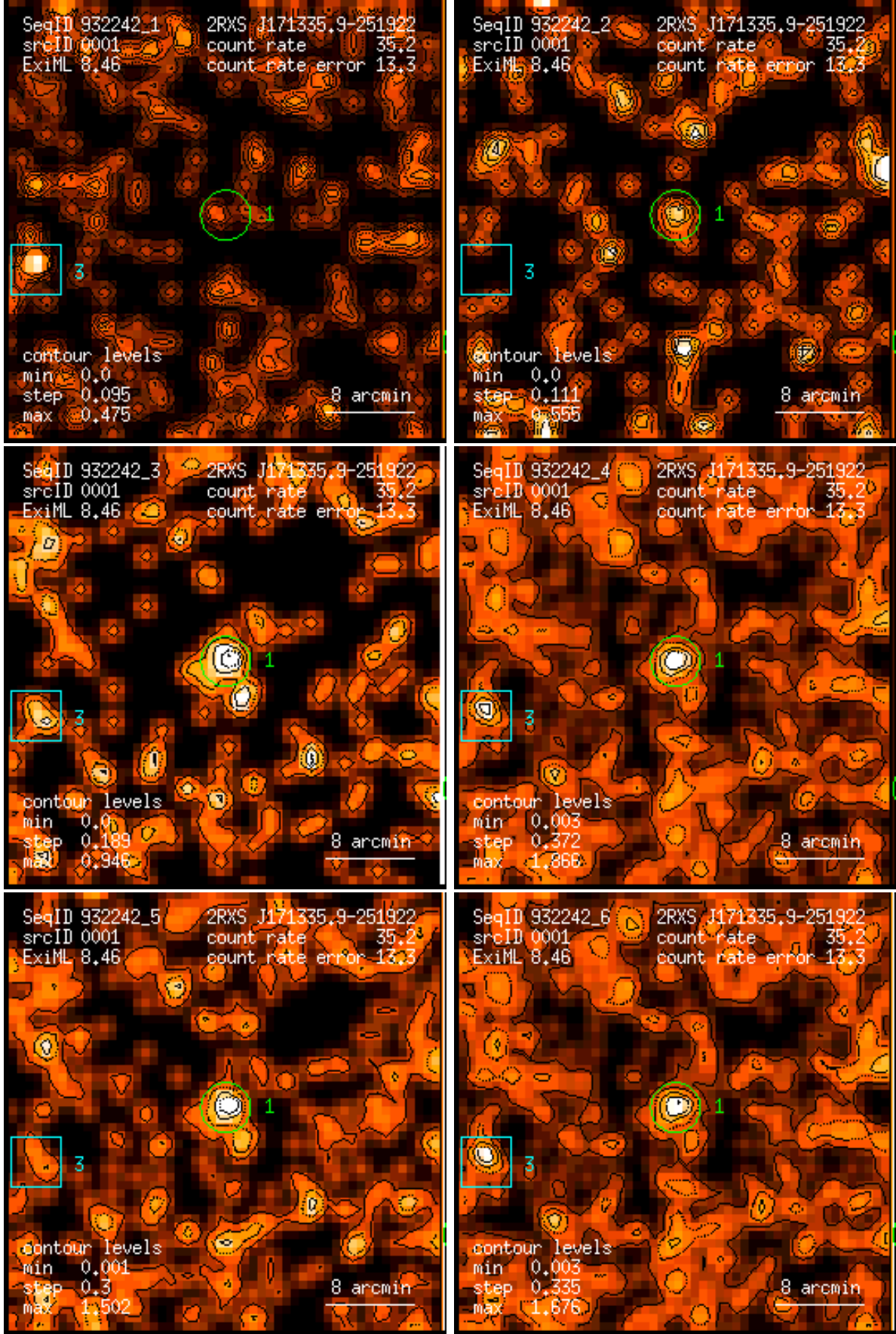
Figure 1: RASS 932242: detection 0001: band rate images, Gaussian filter: (1) PSPC channels 11 – 41, (2) 52 – 90, (3) 91 – 201, (4) 11 – 235, (5) 52 – 201, (6) 11 – 201. Broad band rates in counts/ks. Band rate contour levels in counts/ks/arcmin 2 .
