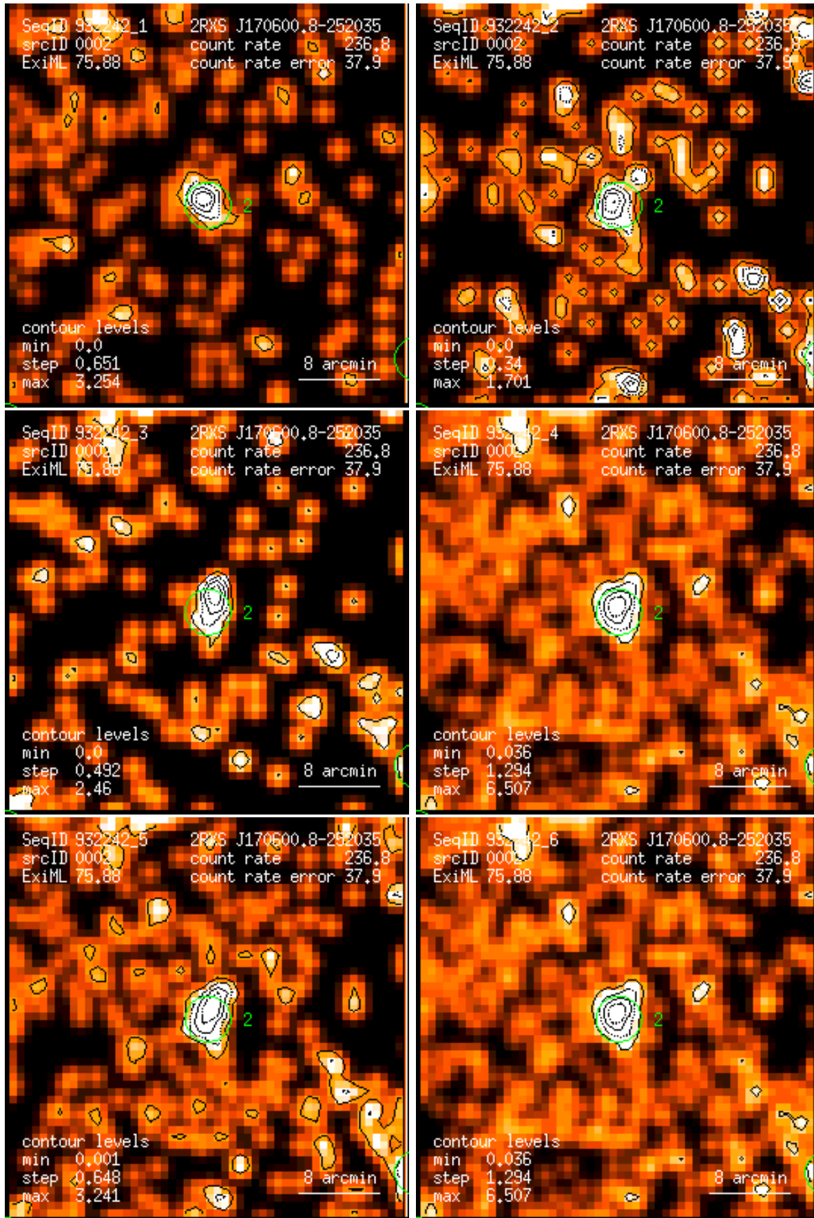
Figure 2: RASS 932242: detection 0002: band rate images, Gaussian filter: (1) PSPC channels 11 – 41, (2) 52 – 90, (3) 91 – 201, (4) 11 – 235, (5) 52 – 201, (6) 11 – 201. Broad band rates in counts/ks. Band rate contour levels in counts/ks/arcmin 2 .
