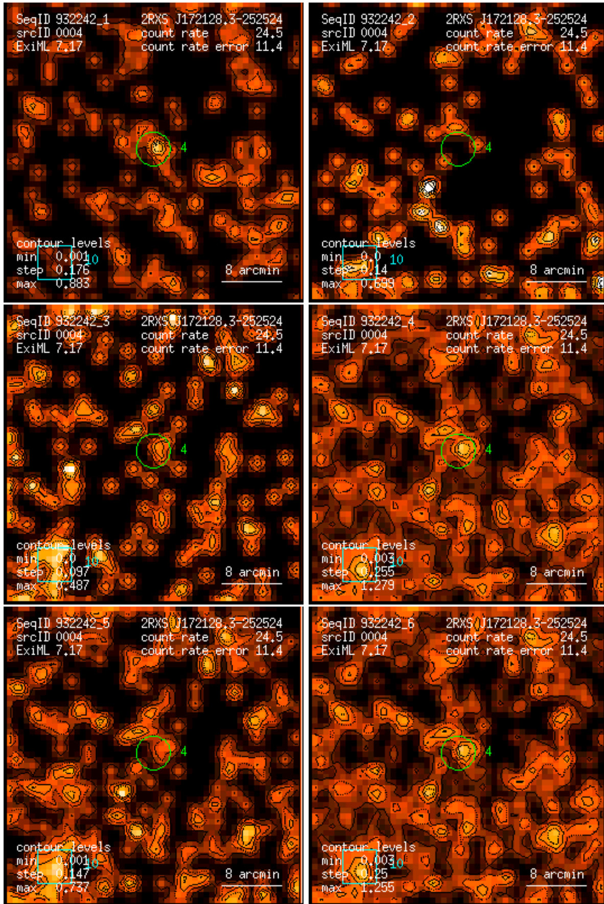
Figure 4: RASS 932242: detection 0004: band rate images, Gaussian filter: (1) PSPC channels 11 – 41, (2) 52 – 90, (3) 91 – 201, (4) 11 – 235, (5) 52 – 201, (6) 11 – 201. Broad band rates in counts/ks. Band rate contour levels in counts/ks/arcmin 2 .
