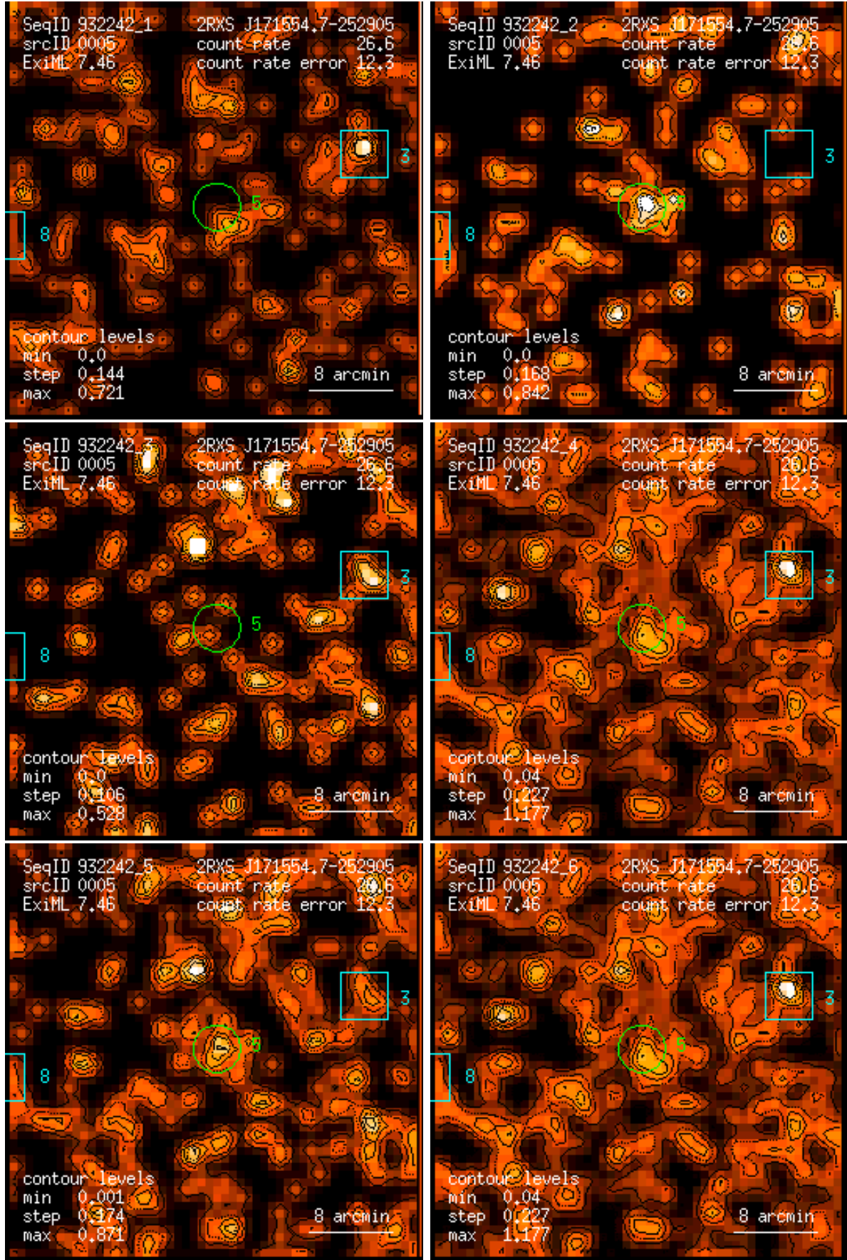
Figure 5: RASS 932242: detection 0005: band rate images, Gaussian filter: (1) PSPC channels 11 – 41, (2) 52 – 90, (3) 91 – 201, (4) 11 – 235, (5) 52 – 201, (6) 11 – 201. Broad band rates in counts/ks. Band rate contour levels in counts/ks/arcmin 2 .
