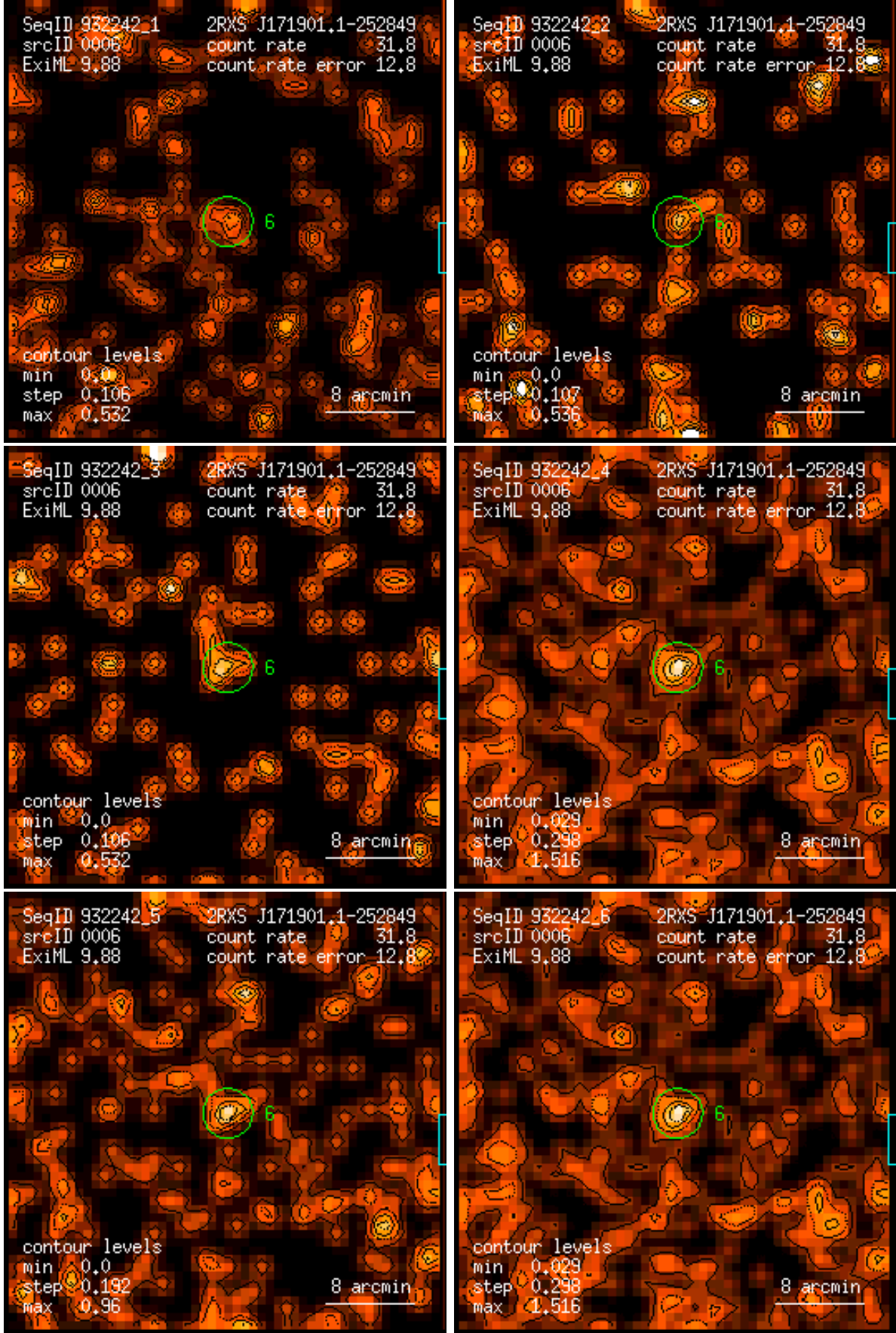
Figure 6: RASS 932242: detection 0006: band rate images, Gaussian filter: (1) PSPC channels 11 – 41, (2) 52 – 90, (3) 91 – 201, (4) 11 – 235, (5) 52 – 201, (6) 11 – 201. Broad band rates in counts/ks. Band rate contour levels in counts/ks/arcmin 2 .
