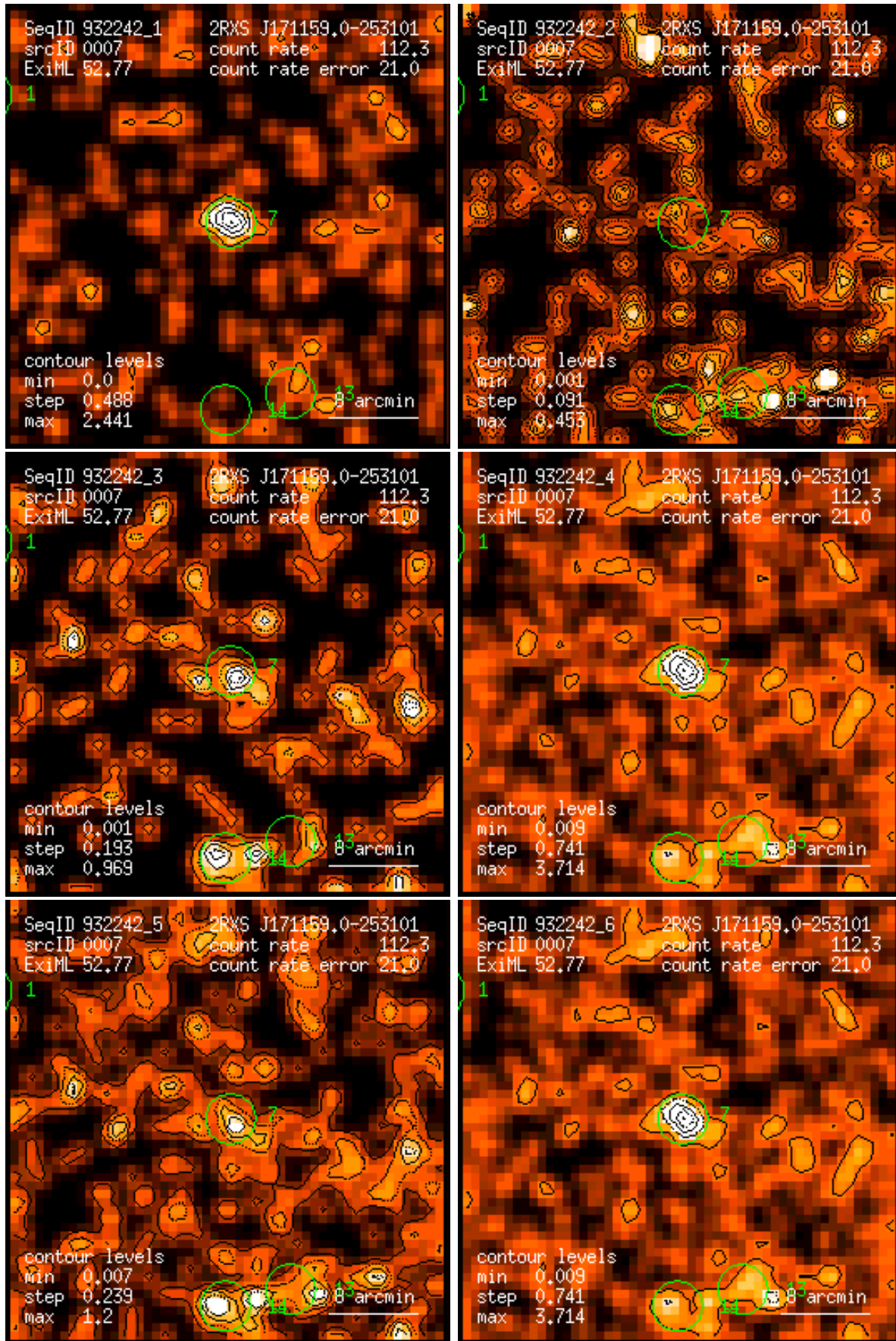
Figure 7: RASS 932242: detection 0007: band rate images, Gaussian filter: (1) PSPC channels 11 – 41, (2) 52 – 90, (3) 91 – 201, (4) 11 – 235, (5) 52 – 201, (6) 11 – 201. Broad band rates in counts/ks. Band rate contour levels in counts/ks/arcmin 2 .
