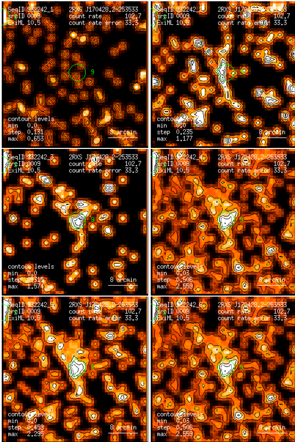
Figure 9: RASS 932242: detection 0009: band rate images, Gaussian filter: (1) PSPC channels 11 – 41, (2) 52 – 90, (3) 91 – 201, (4) 11 – 235, (5) 52 – 201, (6) 11 – 201. Broad band rates in counts/ks. Band rate contour levels in counts/ks/arcmin 2 .
