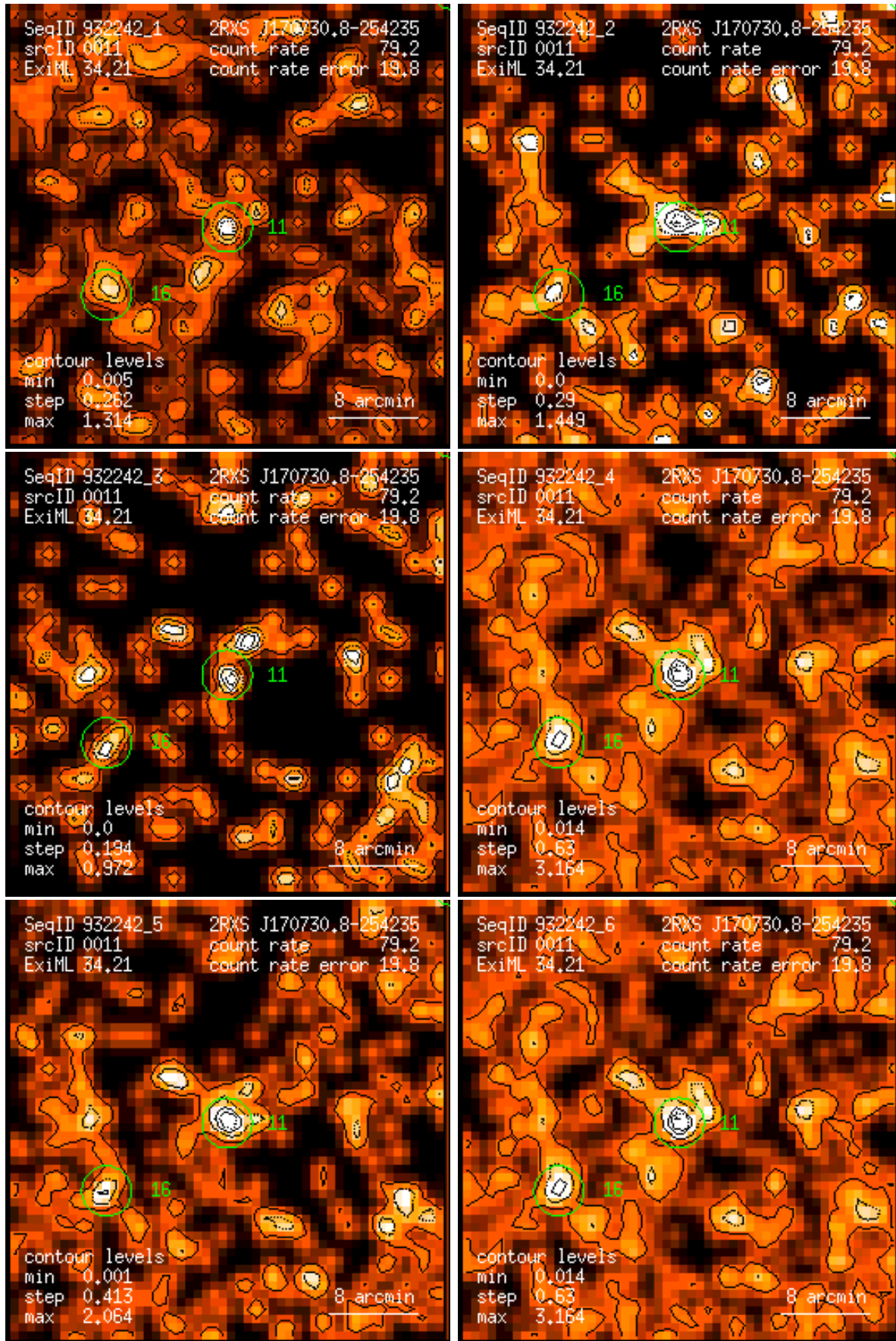
Figure 11: RASS 932242: detection 0011: band rate images, Gaussian filter: (1) PSPC channels 11 – 41, (2) 52 – 90, (3) 91 – 201, (4) 11 – 235, (5) 52 – 201, (6) 11 – 201. Broad band rates in counts/ks. Band rate contour levels in counts/ks/arcmin 2 .
