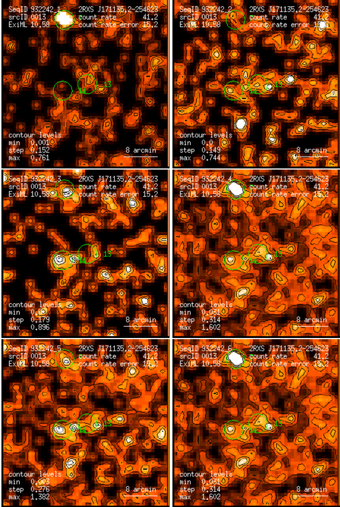
Figure 13: RASS 932242: detection 0013: band rate images, Gaussian filter: (1) PSPC channels 11 – 41, (2) 52 – 90, (3) 91 – 201, (4) 11 – 235, (5) 52 – 201, (6) 11 – 201. Broad band rates in counts/ks. Band rate contour levels in counts/ks/arcmin 2 .
