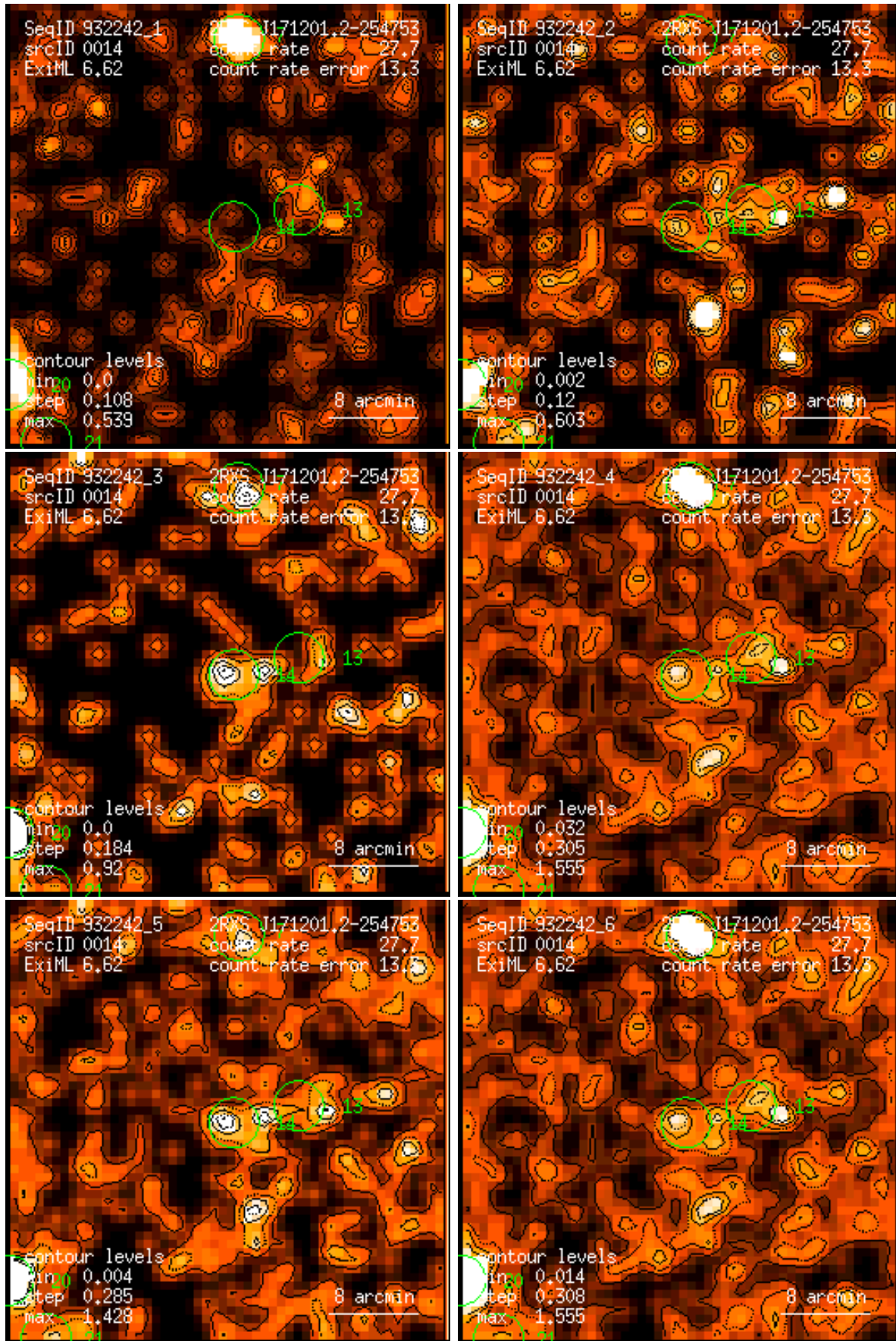
Figure 14: RASS 932242: detection 0014: band rate images, Gaussian filter: (1) PSPC channels 11 – 41, (2) 52 – 90, (3) 91 – 201, (4) 11 – 235, (5) 52 – 201, (6) 11 – 201. Broad band rates in counts/ks. Band rate contour levels in counts/ks/arcmin 2 .
