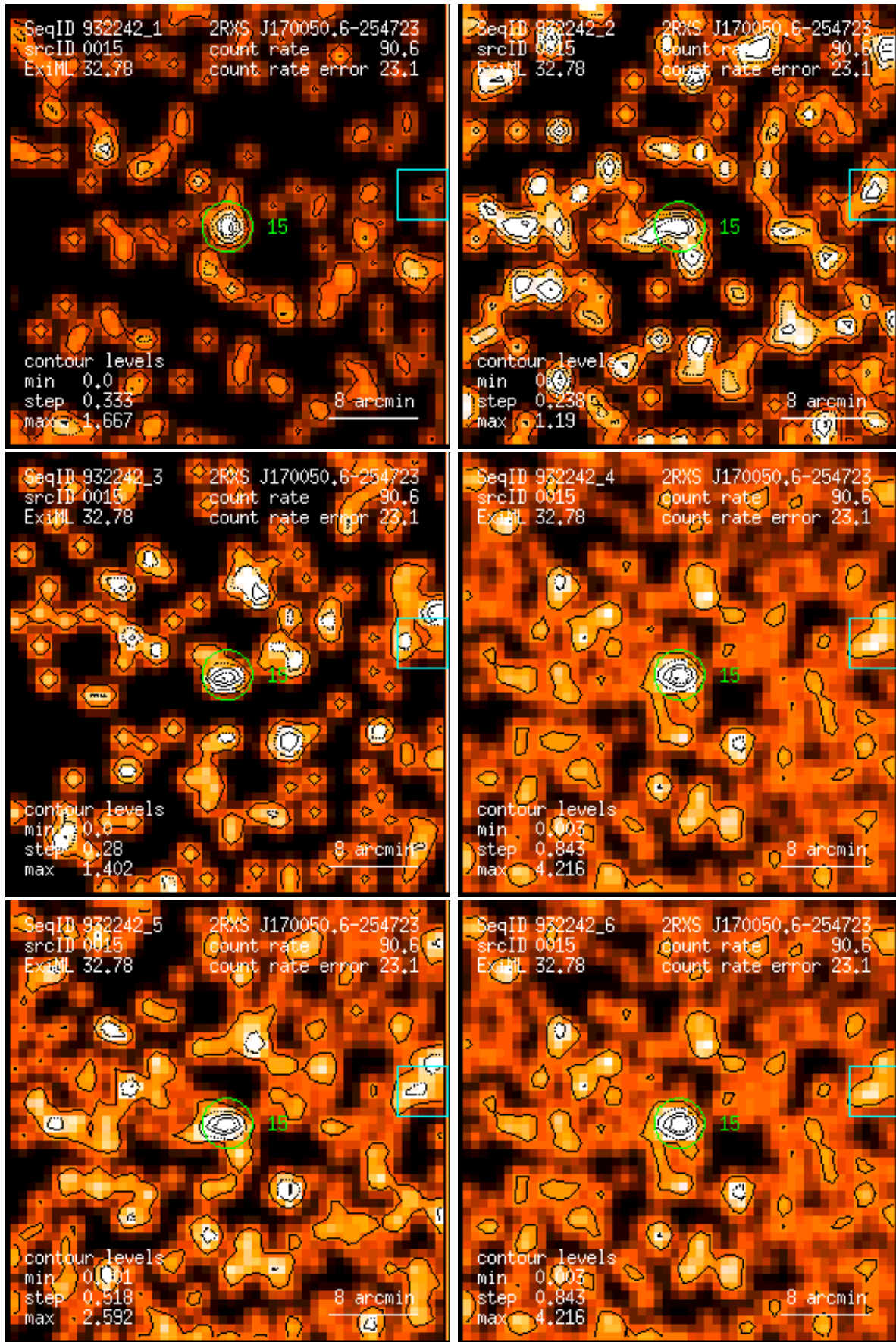
Figure 15: RASS 932242: detection 0015: band rate images, Gaussian filter: (1) PSPC channels 11 – 41, (2) 52 – 90, (3) 91 – 201, (4) 11 – 235, (5) 52 – 201, (6) 11 – 201. Broad band rates in counts/ks. Band rate contour levels in counts/ks/arcmin 2 .
