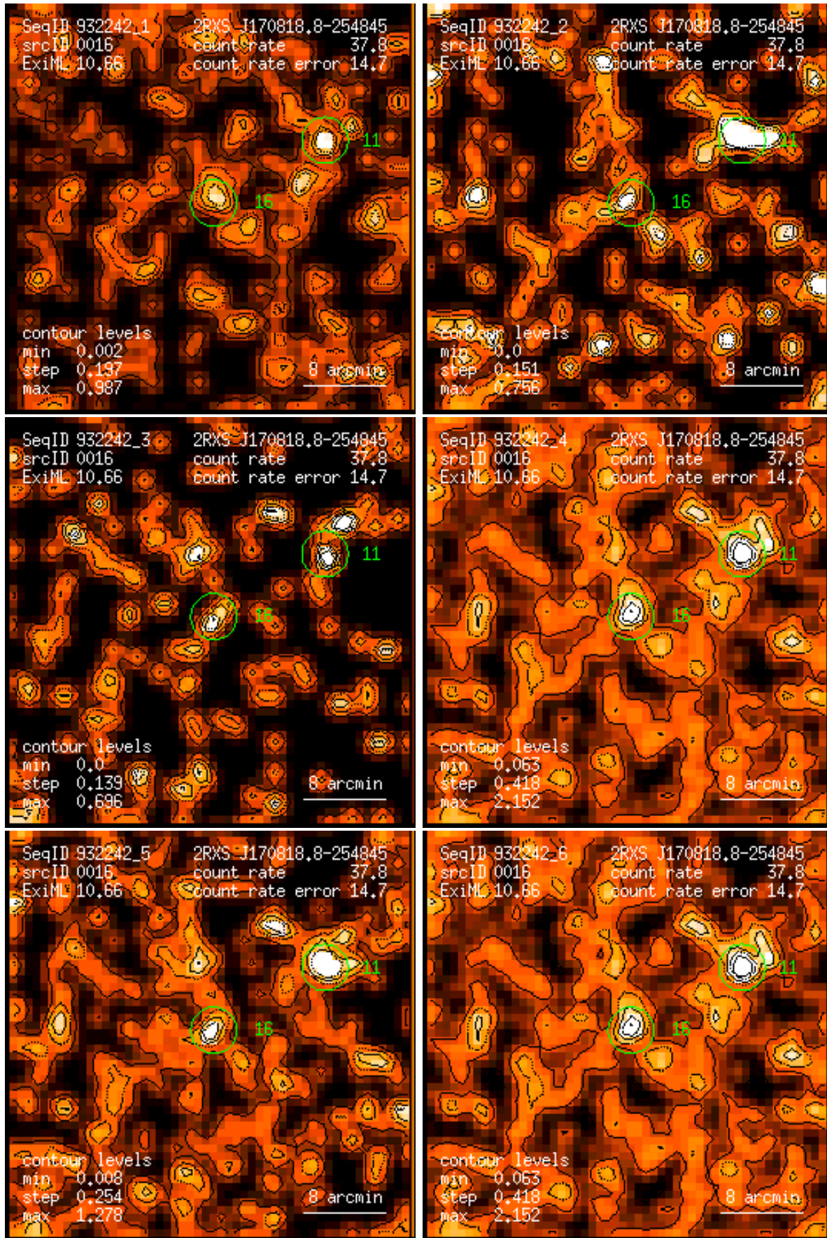
Figure 16: RASS 932242: detection 0016: band rate images, Gaussian filter: (1) PSPC channels 11 – 41, (2) 52 – 90, (3) 91 – 201, (4) 11 – 235, (5) 52 – 201, (6) 11 – 201. Broad band rates in counts/ks. Band rate contour levels in counts/ks/arcmin 2 .
